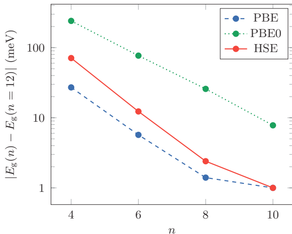
FIG. 3. (Color online) Convergence of the silicon band gap E_g for the functionals PBE (blue, dashed), PBE0 (green, dotted), and HSE (red, solid) with respect to the \mathbf{k} -point mesh ( n \times n \times n ).
