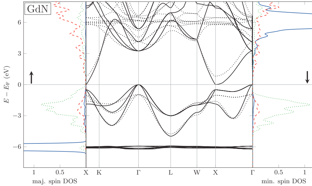
FIG. 4. (Color online) Band structure and density of states (DOS in states per eV) of GdN at the experimental lattice constant. The majority and minority bands are plotted as solid and dotted lines, respectively. The orbital-resolved DOS is shown on the left for majority and on the right for minority states. The solid blue line shows the Gd 4f states, the red dashed line the Gd 5d states, and the green dotted line the N 2p states.
