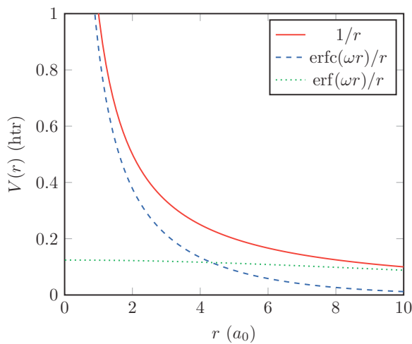
FIG. 1. (Color online) Comparison of the bare (red solid line) and the screened (blue dashed line) Coulomb potentials with the difference between both (green dotted line). The difference does not exhibit a divergence at r = 0 and is a smooth function everywhere. Its Fourier transform converges very rapidly.
