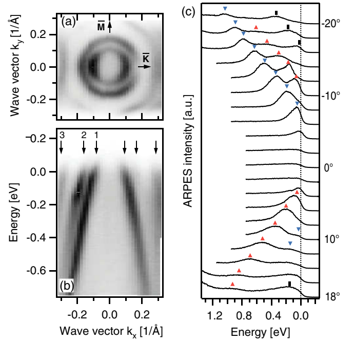
FIG. 2. (Color online) Spin-integrated photoemission from Bi/Cu(111) obtained with Xe I excitation. (a) and (b) show the Fermi surface and the band structure along the \bar{\Gamma}\bar{K} direction. In (c) we display energy distribution curves around \bar{\Gamma} obtained from the same data set as the map in (b).
