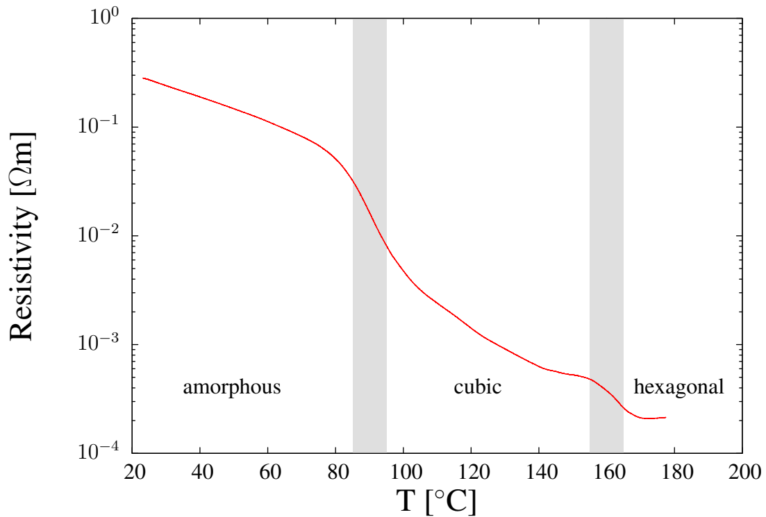
Figure 4.7: Temperature dependent resistivity curve measured on SST. There are two drops of the resistivity at about 85^\circ to 95^\circ\text{C} and 155^\circ to 165^\circ\text{C} which indicate the phase changes from amorphous to cubic and from cubic to hexagonal, respectively.
