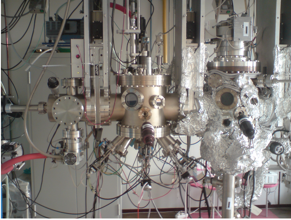
Figure 3.1: A close up of the KOMA-facility. The preparation chamber with the crucibles attached at the bottom is in the center.
