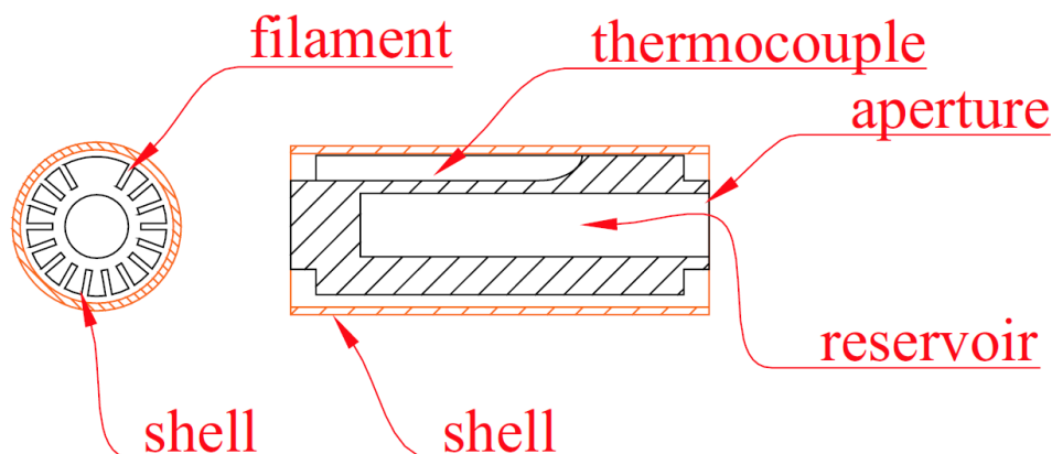
Figure 3.3: The crucible seen from the top (left) and from the front side (right) [9]. It is wrapped by a tantalum filament in order to heat the crucible. The thermocouple is very close to the crucible.
