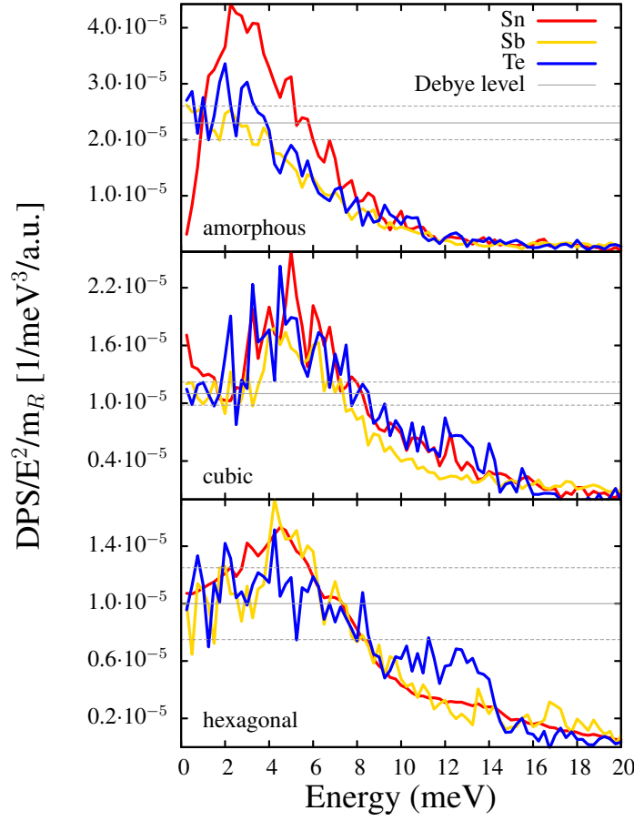
Figure 5.7: Debye level for the amorphous, the cubic and the hexagonal sample. The Debye level is determined until around 3 meV and plotted with the error bar. For the amorphous and the cubic phase Sn was not considered in the determination of the Debye level.
