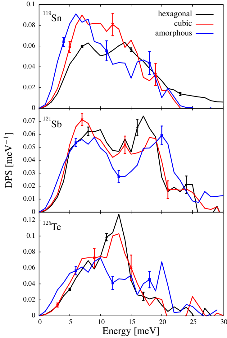
Figure 5.4: The DPS for every isotope of SST. The hardening of the acoustic modes is observed in all three isotopes, however, the vibrational softening of the optical modes just occurs for Sb and Te.
