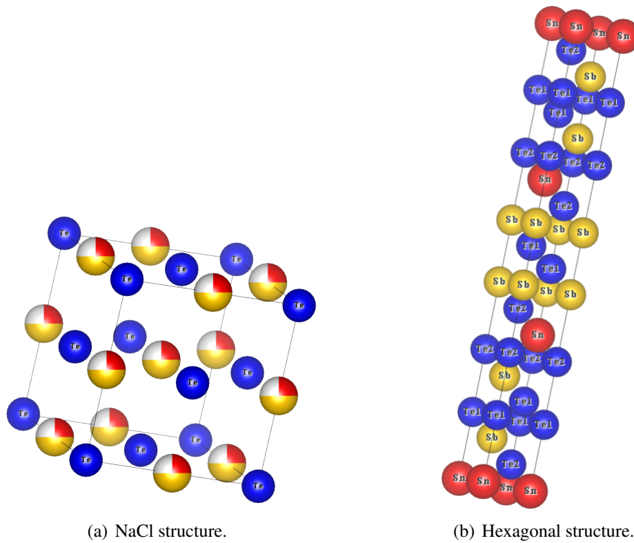
Figure 2.4: Structures of the two crystalline phases of \text{SnSb}_2\text{Te}_4 .
