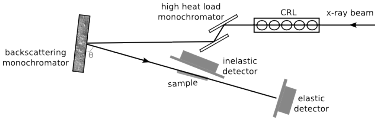
Figure 5.1: Schematic set-up of the beamline applied for nuclear inelastic scattering. The synchrotron radiation beam is monochromatized to the eV range by the high heat load monochromator. The backscattering monochromator further reduces the bandwidth to meV by using a Bragg reflection \Theta > 89.9^\circ . One detector is located close to the sample in order to cover a large angle of the inelastic signal. The second detector far away from the sample records the elastic peak.
