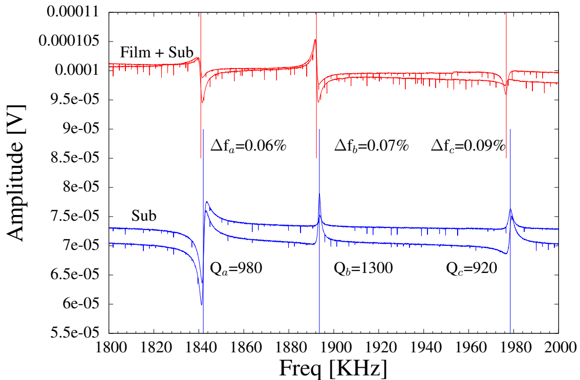
Figure 4.10: Resonance spectra for the substrate and for the substrate with film. There is a small shift of the peaks to lower frequencies in the range of 0.1%. Q indicates the quality factors of the substrate's resonances.
