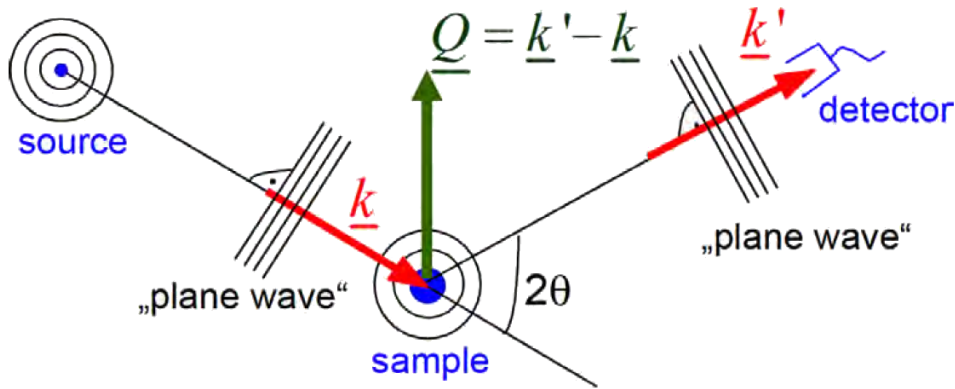
Figure 2.7: Fraunhofer approximation and the scattering vector [15].
