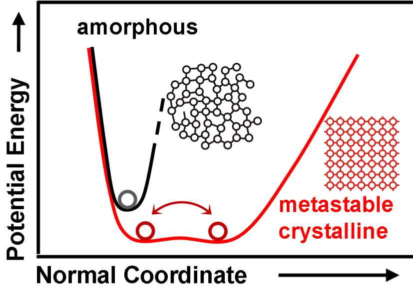
Figure 2.1: Schematic illustration of the potential energies for the amorphous and the cubic phase of an arbitrary PCM. For the amorphous phase the potential is harmonic, however, the potential of the crystalline state exhibits large anharmonicity and more than one energy minimum [8].
