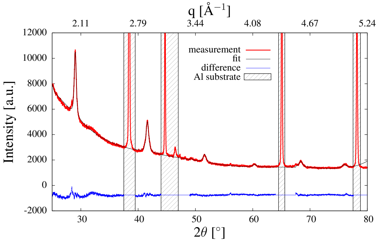
Figure 4.4: Profile matching of the cubic sample. The blue line depicts the residual and the Al peaks are hatched out. The fit (black) is in good agreement with the data (red).
