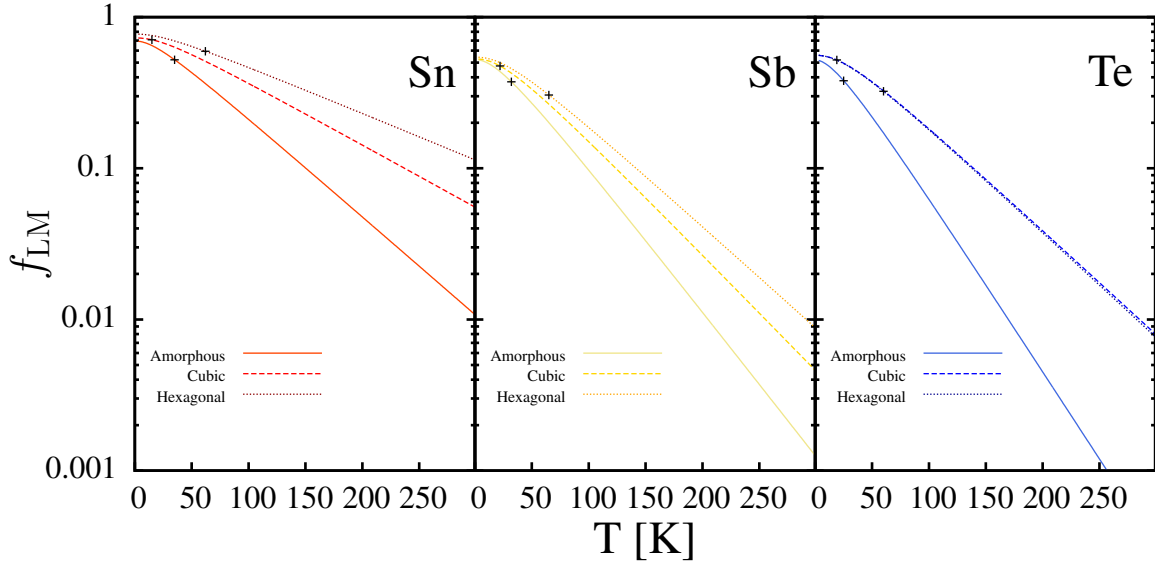
Figure 5.8: Temperature dependence of the Lamb-Mössbauer factor. All f_{\text{LM}} drop by two to three orders of magnitude between 10 and 300 K. For Te the crystalline curves overlap.
