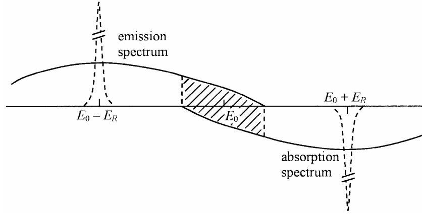
Figure 2.9: Emission and absorption spectra of a photon considering the recoil energy of the nucleus [17]. For a non-moving nucleus the energy of the emitted or absorbed photon has a sharp peak at the energy E_0 - E_R or E_0 + E_R , respectively, whose broadening is just determined by the natural lifetime of the nucleus. The wide solid line indicates the case of a moving nucleus leading to a large Doppler broadening.
