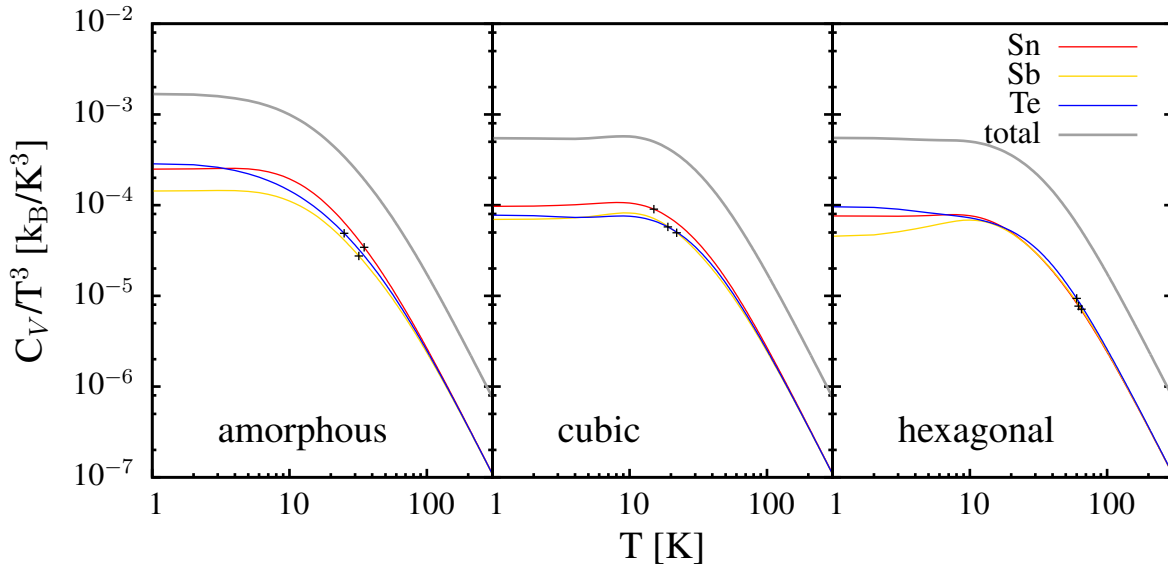
Figure 5.9: Heat capacity at constant volume for the amorphous, cubic and hexagonal phase. The temperature dependence was calculated from the DPS in a harmonic approximation. The total heat capacity is the sum of the partial heat capacities with respect to their relative abundance.
