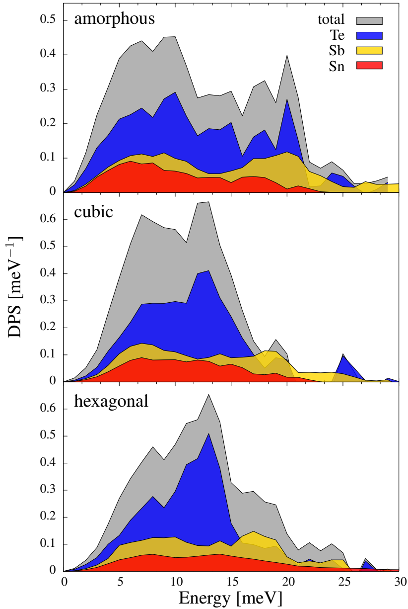
Figure 5.6: Density of Phonon States extracted for all three phases of SST. Each isotope is multiplied by its atomic fraction in the SST compound, the total DPS is calculated by the sum of the partial DPS. The data are plotted up to an energy of 30 meV with a binning of 1 meV. The DPS of hexagonal Sn and the amorphous Sb converge to zero at about 40 meV which is not shown in the diagrams.
