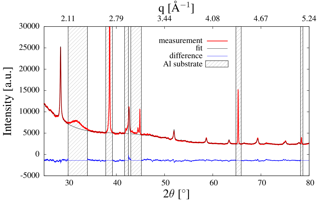
Figure 4.5: Profile matching of the hexagonal sample. The substrate peaks are hatched out. The fit (black) is in good agreement with the data (red). The blue curve represents the difference between measurement and fit.
