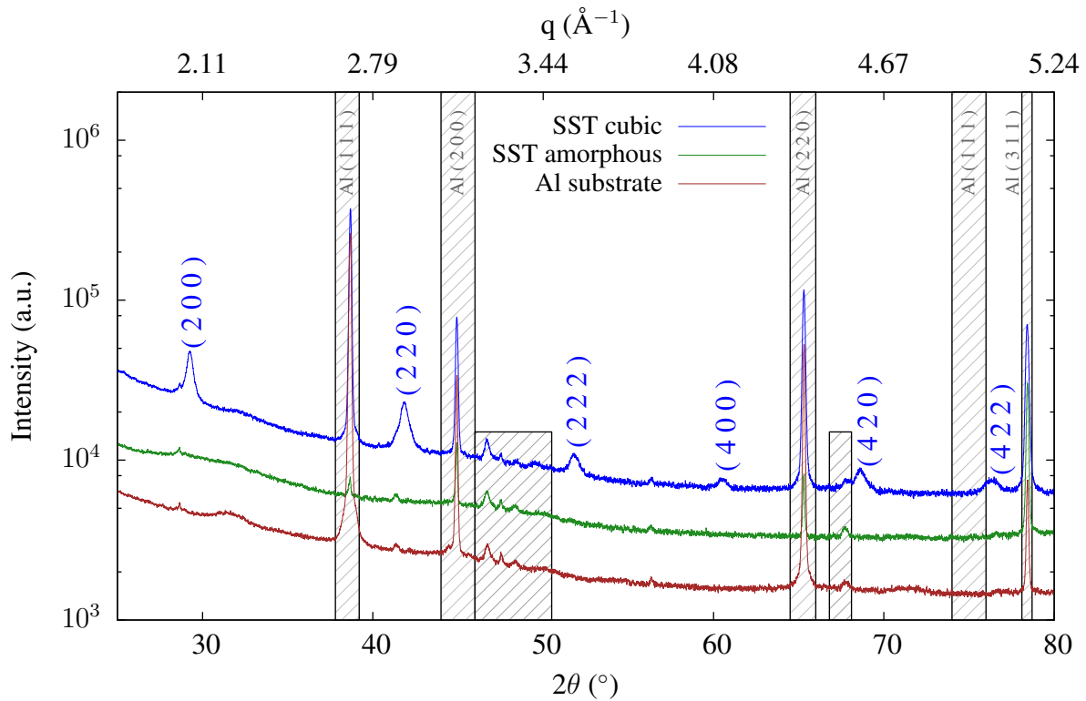
Figure 4.3: XRD measurement of the samples prepared via magnetron sputtering presented in logarithmic scale. The green curve, indicating the as-deposited sample, is purely amorphous. The annealed sample (blue curve) exhibits cubic peaks depicted with their Miller indices, however, revealing a large FWHM.
