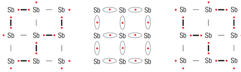
Figure 1.3: A schematic illustration of resonant bonding for a hypothetical simple cubic Sb crystal. On average six Sb atoms share three electrons. The outer pictures show two limiting cases with a shift of electron pairs between the atoms. In reality a superposition of these cases (central picture) is observed leading to a pronounced electron delocalization [7].
