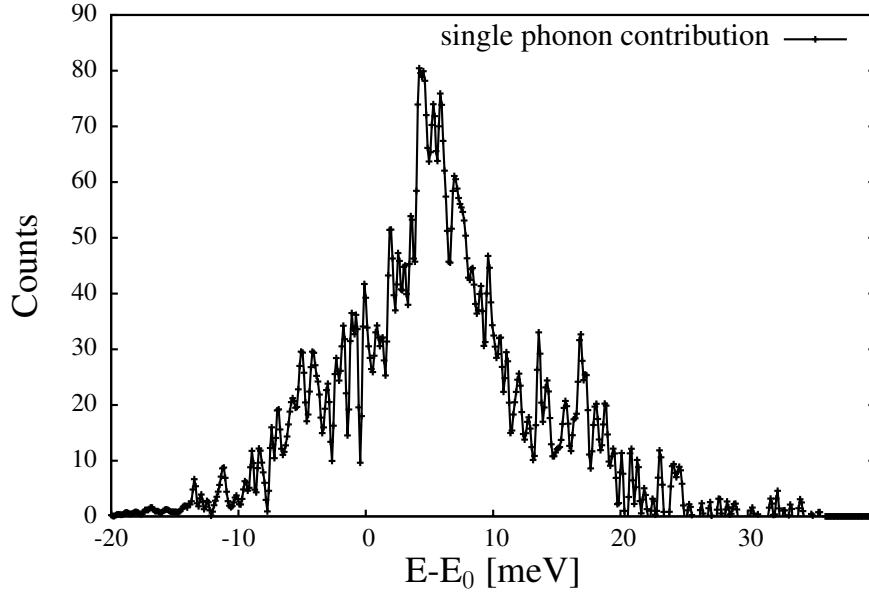
Figure 5.3: The single-phonon contribution extracted from the inelastic spectrum.
