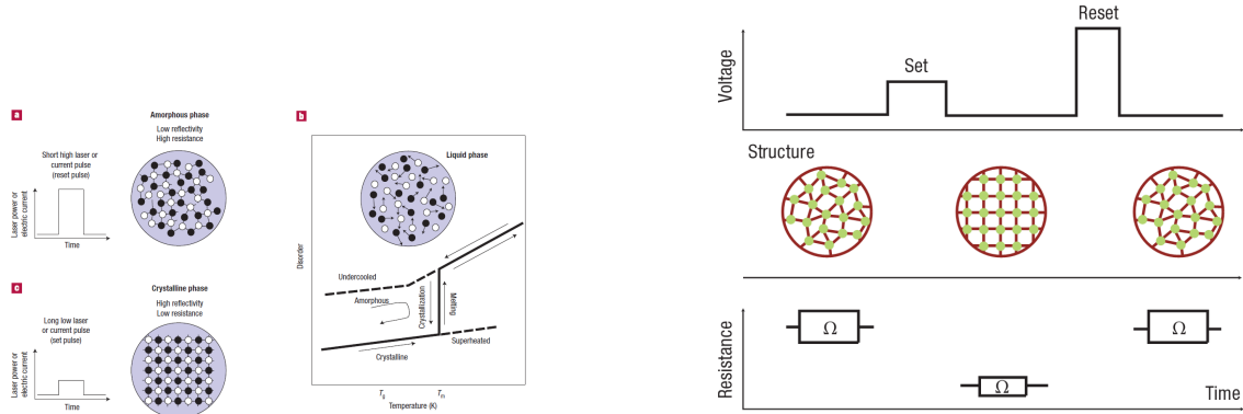
(a) The amorphous material is switched into the crystalline state via laser pulses as it is applied in optical data storages [3].
