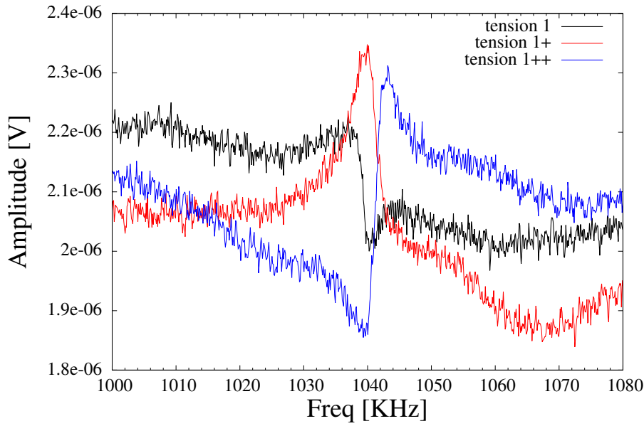
Figure 4.11: Frequency shift due to different loadings of the samples. Different tension of the sample from the transducers leads to a shifting of the frequencies for several kHz.
