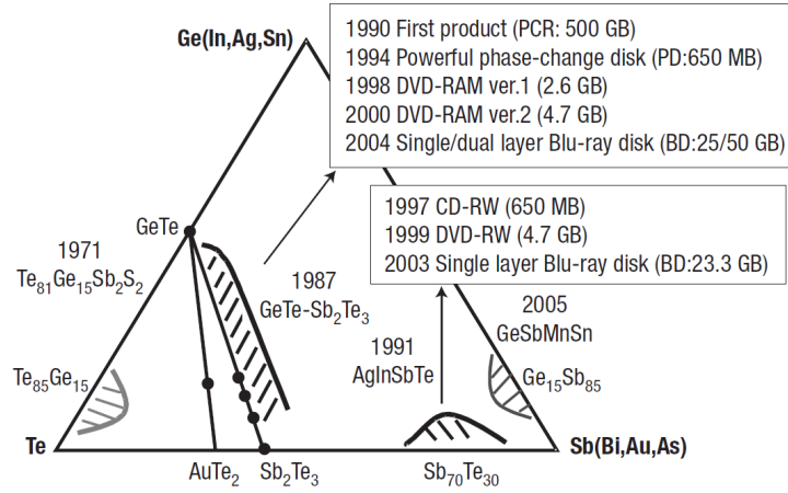
Figure 1.1: Ternary phase change diagram for Te, Sb and Ge [3]. The area between GeTe and Sb_2Te_3 (pseudo binary line) provides many useful PCMs characterized by a large property contrast between the amorphous and the crystalline phase and by low crystallization times.
