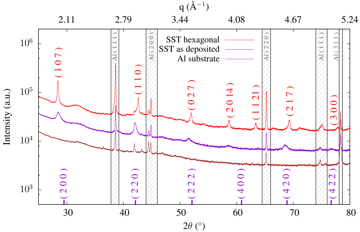
Figure 4.2: XRD measurement of the samples prepared via vapour deposition presented in logarithmic scale. The brown, purple and red curves show the substrate, the as-deposited phase and the hexagonal phase, respectively. The as-deposited sample shows additional peaks with respect to the substrate, hence it is not in the amorphous state. The annealed sample shows a hexagonal structure with all peaks indicated with the corresponding Miller indices.
