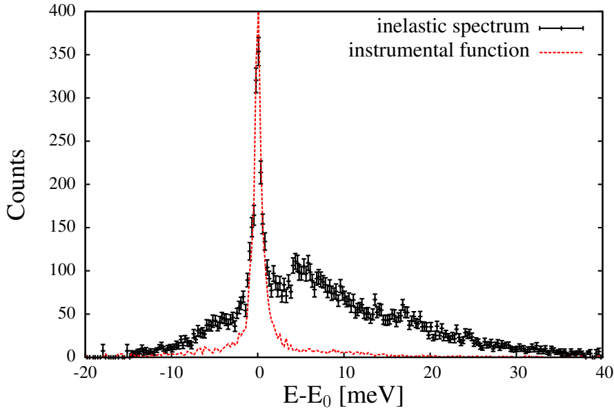
Figure 5.2: Inelastic spectrum (black) and instrumental function (red) of hexagonal SST measured with the ^{121}\text{Sb} resonance.
