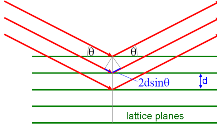
Figure 2.8: The Bragg equation illustrated for a wave scattered at several lattice planes [15].
