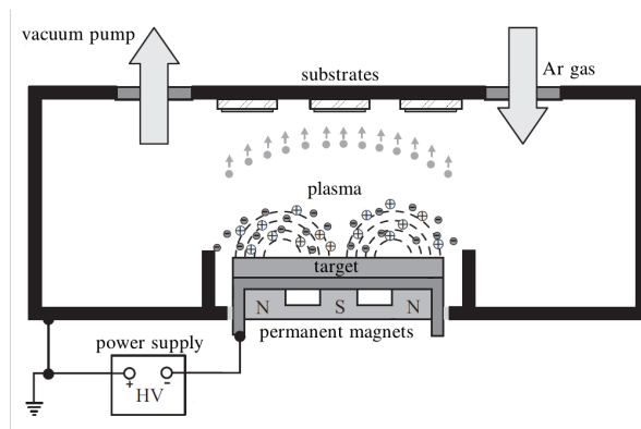
Figure 3.5: A schematic illustration of the magnetron sputtering setup [23]. The Ar gas is ionised by free electrons which are accelerated by the electric field. The Ar-ions produce collision cascades at the target. Neutral target atoms are ejected and distribute inside the chamber.
