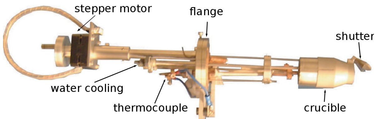
Figure 3.2: The Knudsen cell which was used as evaporation source [9]. The material is located inside the crucible which is opened and closed electronically by a shutter.
