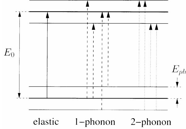
Figure 2.10: Elastic (left) and inelastic scattering processes, the latter accompanied by the creation or annihilation of one (middle) or two phonons (right) [14].
