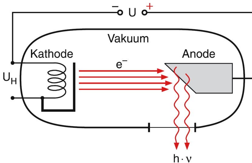
Figure 2.5: Schematic plot of an x-ray tube [13].
