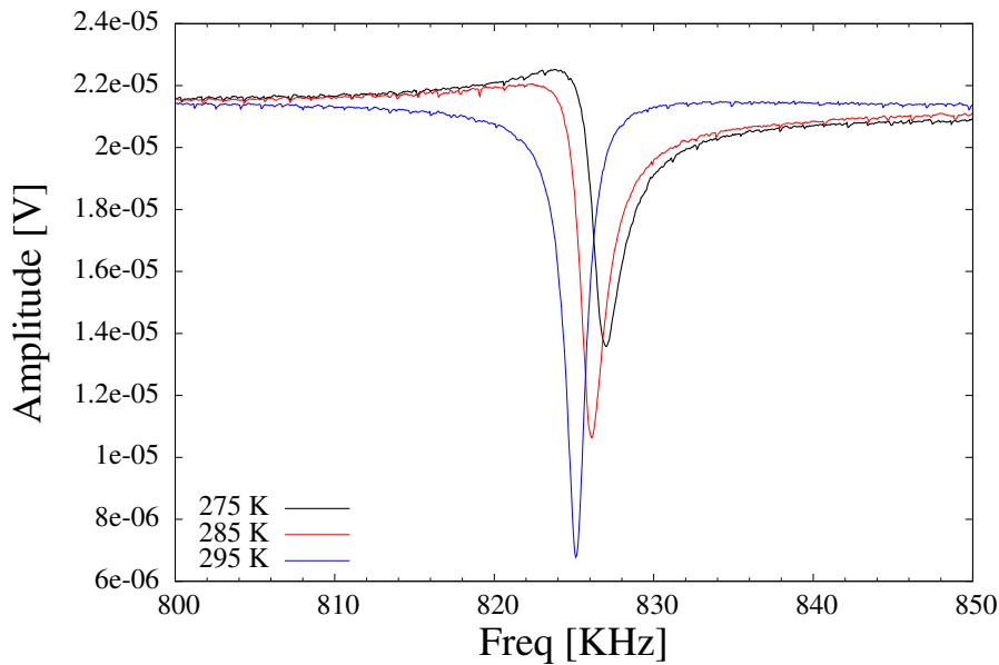
Figure 4.12: Influence of the temperature control upon the resonances of the sample. A variation of ten to twenty Kelvin causes a shift of the frequencies for several kHz.
