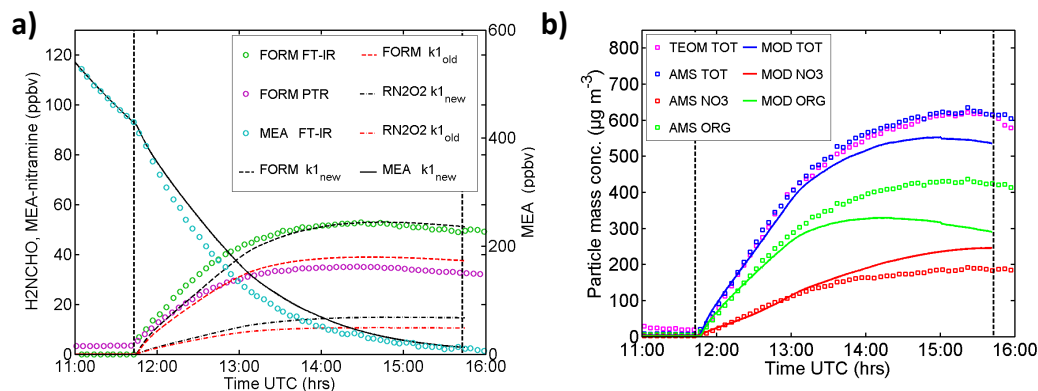
Fig. 5. Concentration time series of experiment E3 on 27 July 2010: (a) measured gas phase concentrations of MEA (FT-IR), formamide (FT-IR and PTR-TOF-MS) and modelled formamide (FORM) and nitramine (RN _2 O _2 ) concentrations using the k(\text{OH} + \text{MEA}) value from EPI Suite v4.0 (red lines) and the value derived in this work (black lines), (b) measured and modelled mass concentrations of nitrate (NO _3 ), high-molecular weight organics >m/z 65 (ORG), and total (TOT) particles. Measured total particle mass data from AMS (blue squares) and TEOM (magenta squares) are in agreement. Nitramine concentrations are scaled by a factor of 5 for better visibility. Vertical dashed lines indicate beginning and end of the sunlit experiment.
