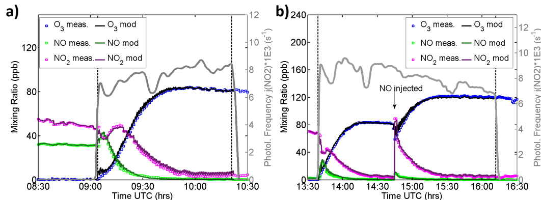
Fig. 1. Measured and modelled time series of \text{O}_3 , \text{NO}_2 , and \text{NO} mixing ratios in (a) experiments E1 and (b) experiment E2. The model was constrained by measured \text{O}_3 , \text{NO}_2 , and \text{NO} concentrations and therefore modelled mixing ratios coincide with measured ones. Photolysis frequency of \text{NO}_2 (scaled by 1 \times 10^3 ) indicated by grey-shaded line. Vertical dashed lines indicate beginning and end of the sunlit experiment.
