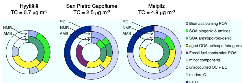
Fig. 6. Source apportionment for TC for Hyytiälä, SPC and Melpitz, based on the different methods used ( ^{14}\text{C} , NMR, AMS).
