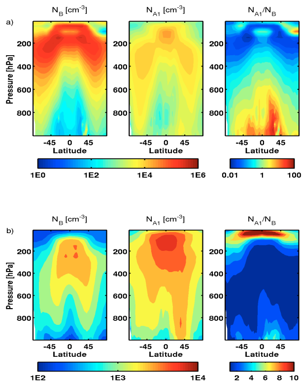
Fig. 14. Annual zonal average concentrations (cm -3 STP (1013.25 hPa, 273.15 K)) of (a) nucleation mode aerosol number; (b) sum of Aitken mode number concentration: centre ones experiment A1 (using activation nucleation in addition to the standard binary nucleation) as predicted by the GCM ECHAM5-HAM; and right panels show the ratio of the yearly averages for experiments B and A1. Notice the different color scales between figures (published in Makkonen et al., 2009).
