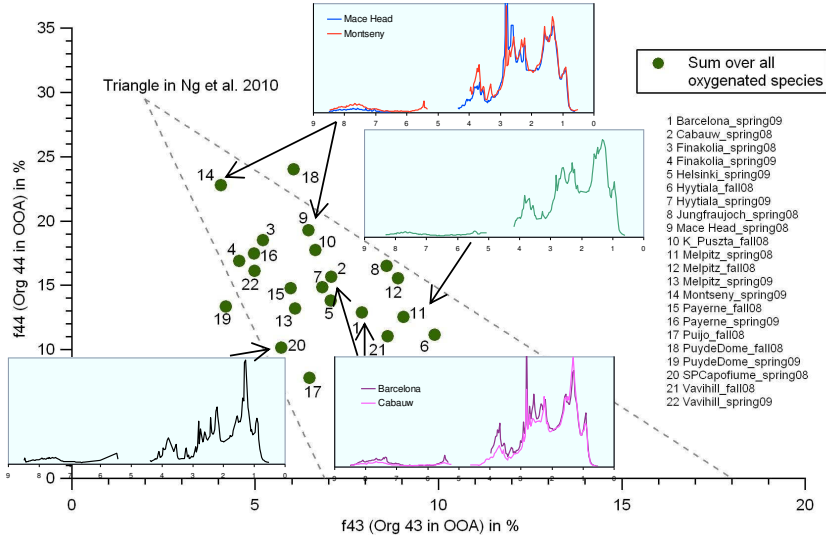
Fig. 7. Average H-NMR spectra from various EUCAARI campaigns compared to the corresponding AMS fingerprints for OOA (Ng et al., 2010). The horizontal axis in the H-NMR spectra reports the chemical shift scale (in ppm). Functional groups are identified based on chemical shift intervals: unfunctionalized alkyls (0.7–1.8 ppm), alkyl groups more (2.5–3.0 ppm) or less (1.8–2.5 ppm) functionalized with carbonyls/carboxyls, hydroxyl (3.3–4.2 ppm) and anomeric (5–6 ppm) groups, and finally aromatics (6–9 ppm).
