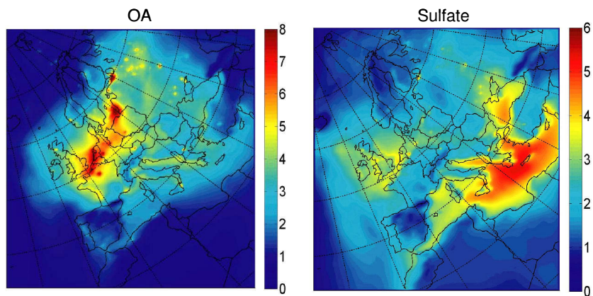
Fig. 19. Ground-level concentration predictions averaged over the entire simulation period (1–29 May 2008) for \text{PM}_{2.5} total organic aerosol and sulfate (in \mu\text{g m}^{-3} ). Different scales are used.
