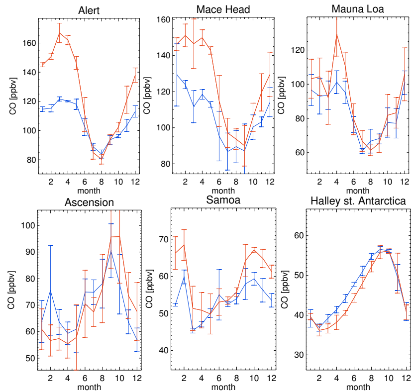
Fig. 3. Monthly mean comparison of TM5 surface CO (blue) against GMD surface observations (red) using co-located model output for 2006, sampled at the measurement times. The error bars indicate the standard deviation in the monthly means.
