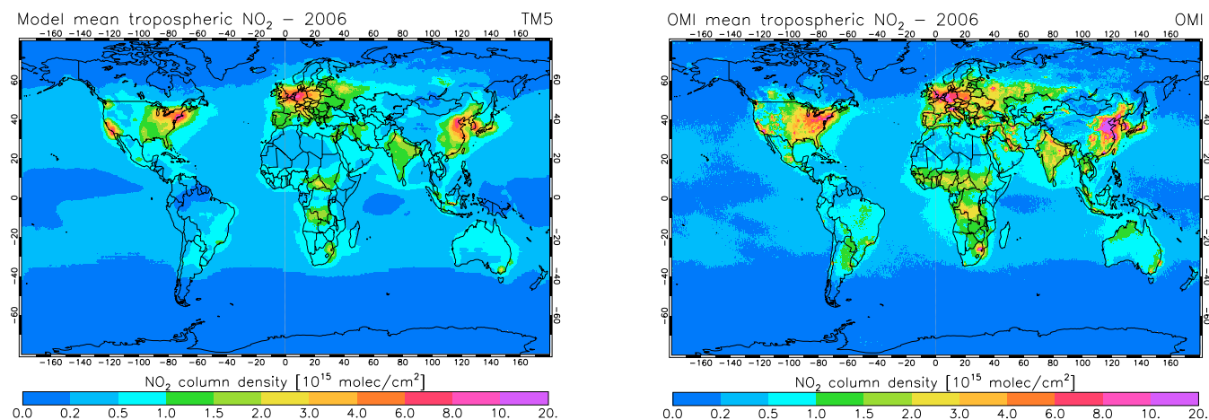
Fig. 9. TM5 annual mean tropospheric \text{NO}_2 column density versus OMI.
