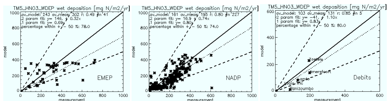
Fig. 13. Scatter plots of the simulated \text{HNO}_3 wet deposition versus measurements for three networks in Europe (left panel), North America (middle panel), and Africa (right panel). Dashed lines have slopes equal to 2 resp. 0.5. The dotted line is the result of linear regression fitting through the origin.
