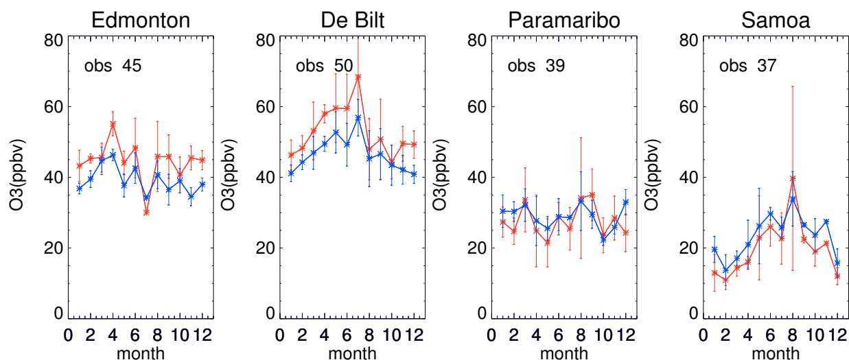
Fig. 15. The annual cycle in the simulated ozone concentrations (blue) in the layers between 800–700 hPa compared to WOUDC sonde observations (red) at the stations Edmonton (53.5° N, 114° W), De Bilt (52° N, 5.2° E), Paramaribo (5.9° N, 55.2° W), and Samoa (14° S, 170.5° W). Model data is sampled at the time of the observations. The error bars indicate the standard deviation in the monthly means.
