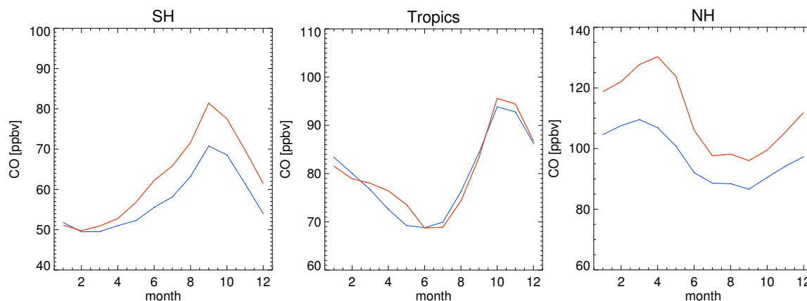
Fig. 5. The annual cycle of mean, mass weighted CO in observations (red) and in TM5 (blue) for the MOPITT 500-hPa retrieval level.
