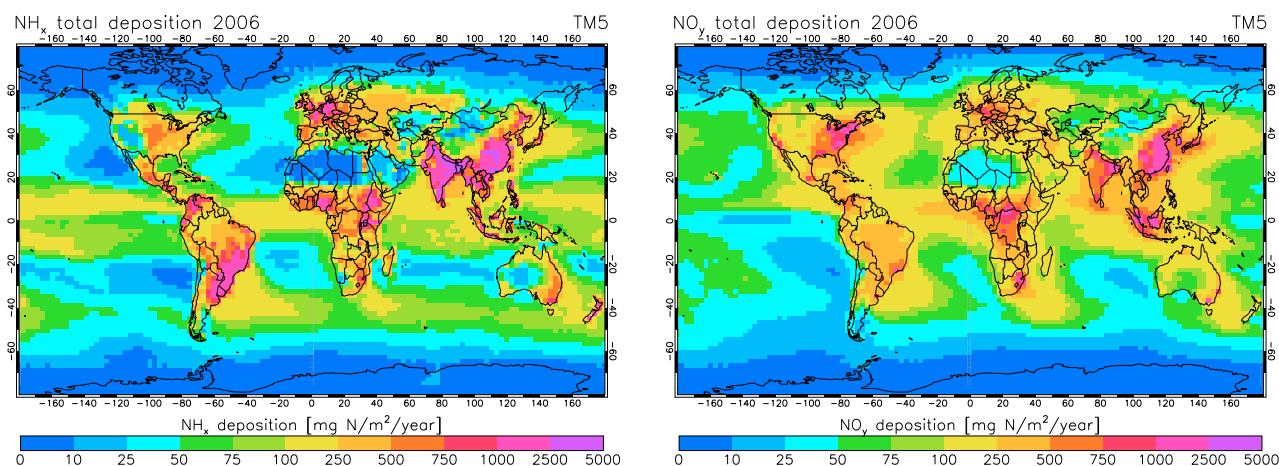
Fig. 12. Annual \text{NH}_x and \text{NO}_y dry and wet deposition in TM5 for 2006.
