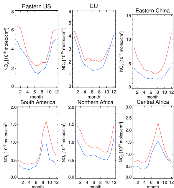
Fig. 10. Annual cycle of regionally and monthly averaged \text{NO}_2 tropospheric columns from TM5 (blue) against OMI (red).
