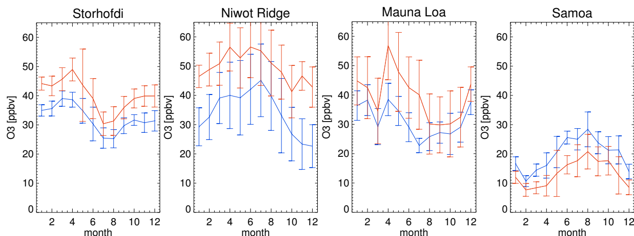
Fig. 14. The annual cycle in the simulated ozone concentrations (blue) compared to surface measurements from the GMD network (red) at the stations Storhofdi, Iceland (63.3° N, 20.3° W), Niwot Ridge (41.1° N, 124.2° W), Mauna Loa (19.5° N, 155.6° W), and Samoa (14° S, 170.5° W). Model data has been sampled at the time of the observations. The error bars indicate the standard deviation in the monthly means.
