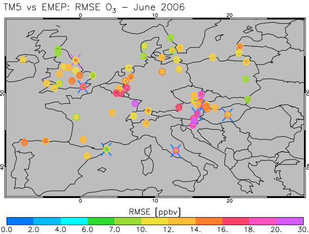
Fig. B2. Root mean square error (RMSE) of modeled surface ozone against hourly EMEP station data at stations below 800 m altitude. Outer circles: 3° × 2° run, middle circles: 1° × 1°, inner circles: 0.5° × 0.25°. Blue crosses denote locations where an increase in resolution leads to a consistent reduction in RMSE with more than 2 ppbv for both zoom runs, compared to the 3° × 2° run. Purple crosses denote a similar consistent increase in RMSE.
