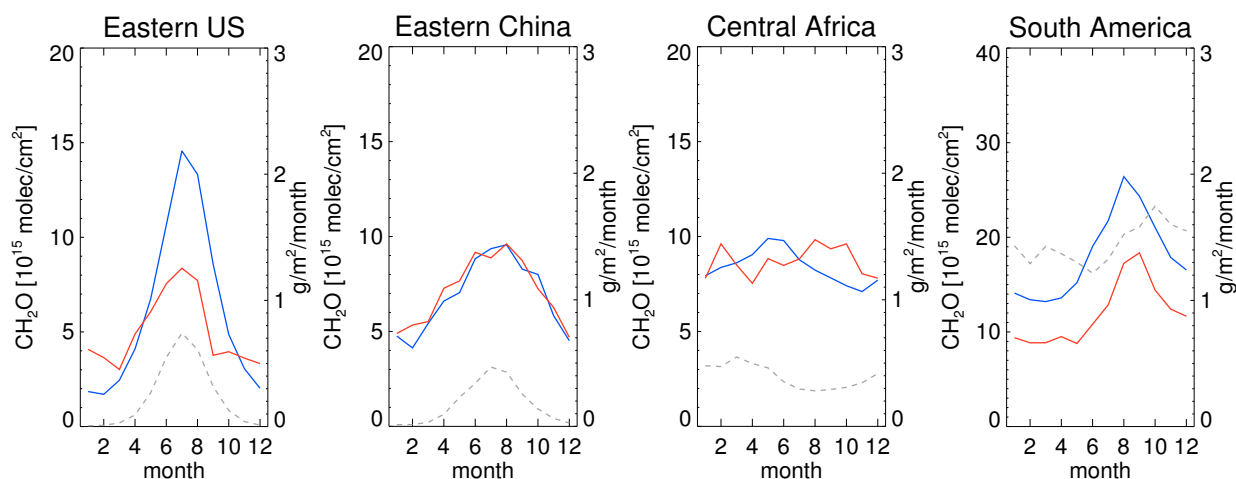
Fig. 8. The annual cycle in the observed (SCIAMACHY, red) and modeled (blue) \text{CH}_2\text{O} tropospheric columns at 10:30 h LT over four selected regions. Dashed lines in grey indicate the isoprene emission flux in \text{g/m}^2/\text{month} . Note the different scale for the columns over South America.
