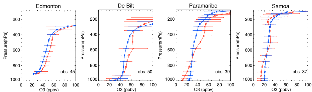
Fig. 16. The annual average modeled ozone profiles (blue) compared to WOUDC sonde observations (red) for the stations shown in Fig. 15.
