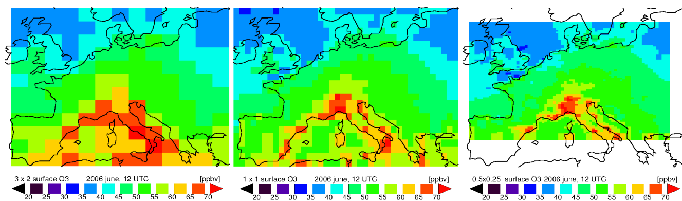
Fig. B1. Monthly mean surface ozone fields over Europe for June 2006 at 12:00 UTC, as simulated with increasing levels of zoom.
