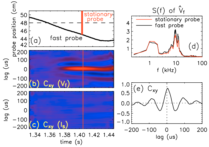
Fig. 1 Long-distance cross-correlation of edge fluctuations in an ohmic discharge (#108272). Time history of (a) fast/stationary probe (dashed line denotes limiter position); (b) contour-plot of C_{xy} on V_f signals; (c) contour-plot of C_{xy} on I_s signals. (d) Power spectrum of V_f fluctuations at the maximum C_{xy} location; (e) cross-correlation of V_f fluctuations at the maximum C_{xy} location.
