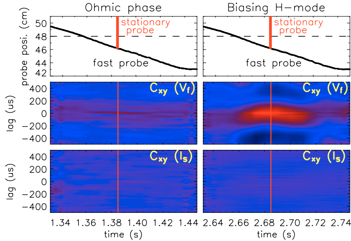
Fig. 2 Time history of fast/stationary probes and the contour-plot of cross-correlation between V_f (middle panels) and I_s (bottom panels) fluctuations measured before (left column) and during (right column) the biasing H-mode (# 108288). The vertical red lines in contour-plots denote the time when the two probes are at the same radial location.
