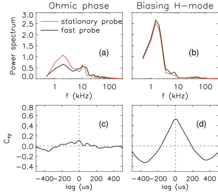
Fig. 3 Power spectrum of V_f fluctuations detected by fast and stationary probes at the maximum C_{xy} location in (a) ohmic and (b) biasing H-mode phase. The corresponding cross-correlation ( C_{xy} ) of V_f measured in (c) ohmic and (d) biasing H-mode phase.
