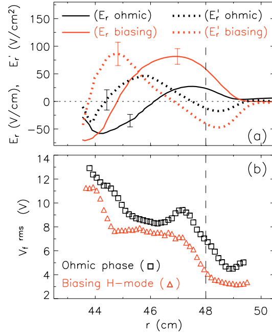
Fig. 4 Radial profiles of (a) E_r and E_r shear ( E_r' ); and (b) the RMS levels of V_f fluctuations before (ohmic) and during the biasing H-mode phases. The vertical dashed line denotes limiter position. The error bars in E_r and E_r' indicate the standard deviation about the mean for similar discharges.
