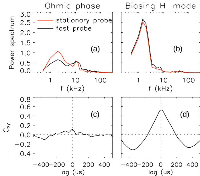
Fig. 3 Power spectrum of V_f fluctuations detected by fast and stationary probes at the maximum C_{xy} location in (a) ohmic and (b) biasing H-mode phase. The corresponding cross-correlation ( C_{xy} ) of V_f measured in (c) ohmic and (d) biasing H-mode phase.
