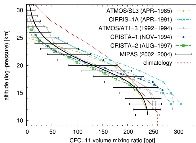
Fig. 9. Comparison of mean CFC-11 vertical profiles from different space experiments. Analysis is restricted to mid-latitude measurements (20 to 65° N/S). Trends are corrected for by mapping all data to the middle of year 2003. For references of data sets see text.
