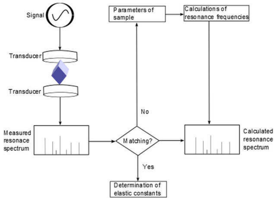
Figure 3.4: Schematic diagram of the RUS measurement and the fitting procedure of the elastic moduli. It is inspired by [20].
