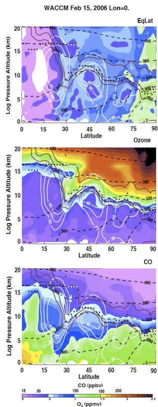
Fig. 8. WACCM NH meridional cross sections of EqLat (top), Ozone (middle) and CO (bottom) for 15 February 2006 along 0° longitude. In each panel, selected meteorological variables are also shown, including isentropes (black dash lines), wind speed (white lines), PV (red lines), and the thermal tropopause (black dots). White color-filled areas of EqLat represent negative values.
