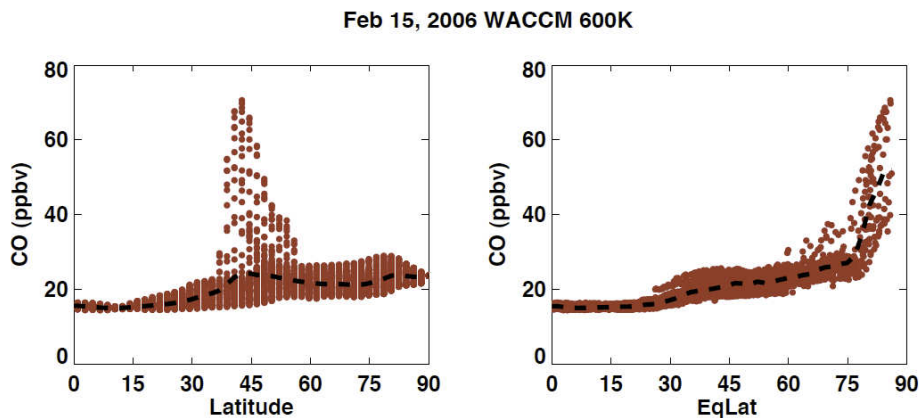
Fig. 4. Scatterplots of WACCM CO at 600 K as functions of latitude (left) and equivalent latitude (right). The black dashed lines represent the zonal means (calculated in 1.9° intervals) in latitude or EqLat coordinates, respectively.
