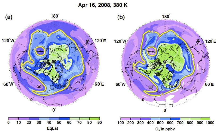
Fig. 10. Maps of (a) EqLat and (b) ozone from the SD-WACCM run for 16 April 2008 at the 380 K potential temperature surface. The 6 puv PV contours are shown by the yellow lines. The dynamical tropopause is defined as the greater 6 puv contour.
