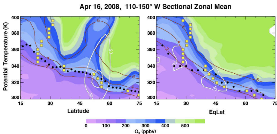
Fig. 12. Sectional zonal means of ozone for 110°–150° W in (a) latitude and (b) EqLat. Yellow squares represent the dynamical tropopause at each isentrope. Black dots represent the thermal tropopause. Also shown are PV in pvu (red contours) and zonal wind in \text{m s}^{-1} (white contours).
