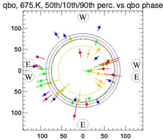
Figure 6. Polar plot of ascent vs. QBO phase. The radii of the circles give the mean ascent of the 675-K air parcels as in Figure 5a over the course of 90 days in K. The black one stands for the climatological average of all starts over the 7 years and colors distinguish between seasons as in Figure 5. Marks with bars stand for the individual trajectory runs and are plotted at the QBO phase at the start of the trajectory calculations. They give the median and 10th/90th percentiles of the vertical distribution at day 90. The QBO phase is rotating counterclockwise and is westerly on the positive ordinate.
