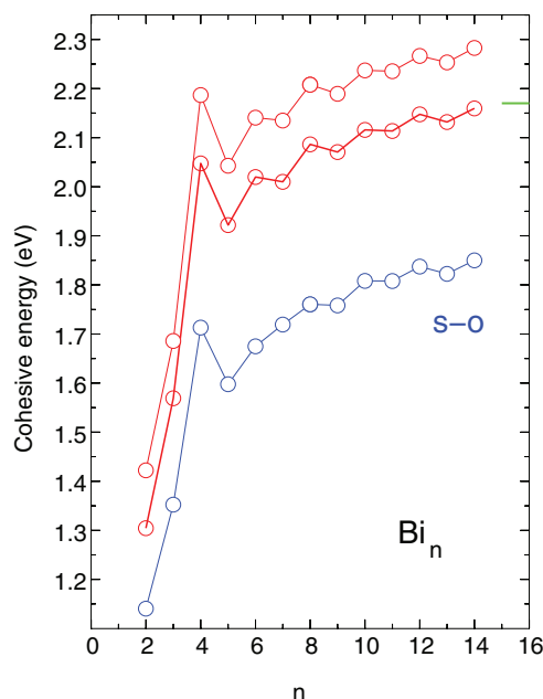
FIG. 5. Cohesive energies of \text{Bi}_n clusters for CPMD-optimized geometries. Thick red: CPMD calculations (no s-o coupling), thin red: VASP calculations (no s-o coupling), blue: VASP calculations (s-o coupling), green: experimental cohesive energy of Bi (Ref. 58).
