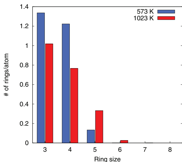
FIG. 11. Ring distributions in liquid Bi at 573 and 1023 K.
