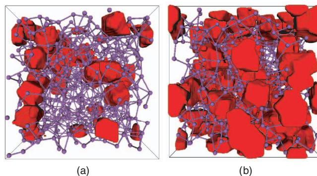
FIG. 7. Snapshots of liquid Bi at (a) 573 K and (b) 1023 K. The cavities are shown in red.
