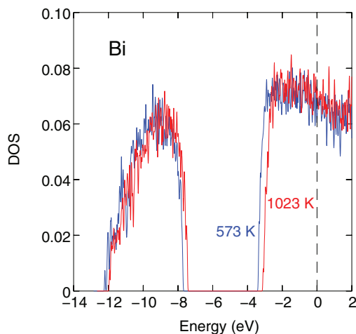
FIG. 14. Electronic density of states for liquid Bi at T = 573 K (blue) and 1023 K (red). The Fermi energy (dashed) is zero in each case.
