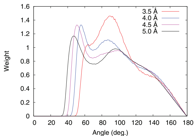
FIG. 10. Bond angle distribution at 573 K as a function of cutoff distance.
