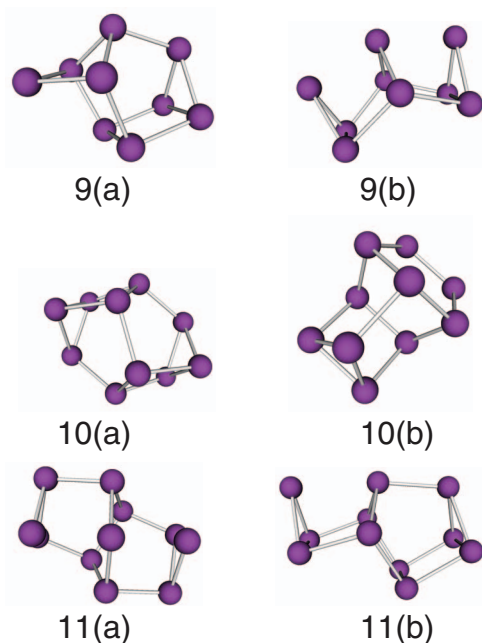
FIG. 3. Isomers of \text{Bi}_9 , \text{Bi}_{10} , and \text{Bi}_{11} . (a) denotes the most stable isomer, (b) the next highest in energy.
