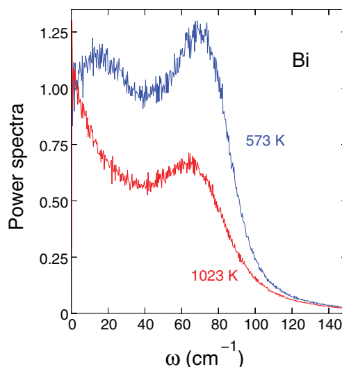
FIG. 13. Calculated power spectra for liquid Bi at 573 K (blue) and 1023 K (red). Curves are normalized to unity at zero frequency.
