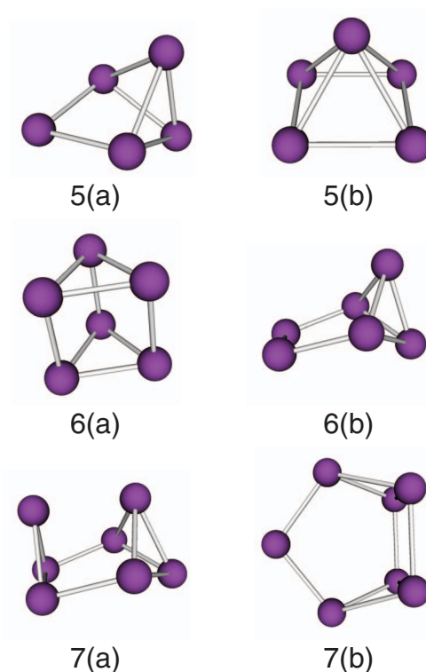
FIG. 1. Isomers of Bi 5 , Bi 6 , and Bi 7 . (a) denotes the most stable isomer, (b) the next highest in energy.
