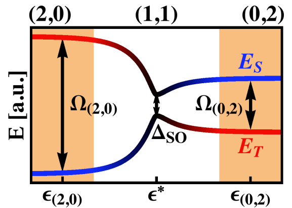
FIG. 3. (Color online) Sketch of the energy levels |S\rangle and |T\rangle that encode the ISTQ. The energy levels are shifted compared to Fig. 2, while the energy differences between E_S and E_T remain unchanged at each \epsilon . |S\rangle and |T\rangle have equal orbital energies at \epsilon^* . SOIs lift the degeneracy and cause an anticrossing \Delta_{\text{so}} . |S\rangle is the ground state for \epsilon < \epsilon^* , but |S\rangle is the excited state for \epsilon > \epsilon^* . We label one point deep in (2,0) by \epsilon_{(2,0)} with the energy splitting \Omega_{(2,0)} [similarly, |S\rangle and |T\rangle have the energy splitting \Omega_{(0,2)} at \epsilon_{(0,2)} in (0,2)].
