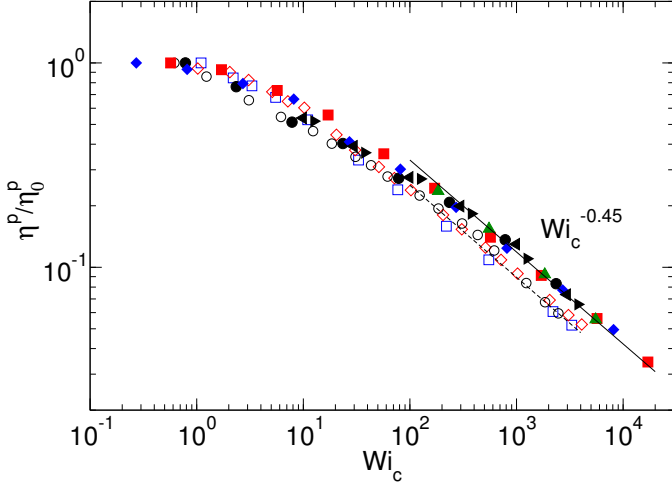
Figure 4: Dependence of the polymer contribution to shear viscosity on Wi_c . Open symbols correspond to systems of polymer length N_m = 50 for c/c^* = 0.16 ( \circ ), c/c^* = 1.6 ( \diamond ), and c/c^* = 2.08 ( \square ). Filled symbols denote results for N_m = 250 with the concentration c/c^* = 0.17 ( \bullet ), c/c^* = 0.35 ( \blacktriangle ), c/c^* = 1.38 ( \blacktriangleright ), c/c^* = 2.77 ( \blacktriangleup ), c/c^* = 5.19 ( \blacklozenge ), and c/c^* = 10.38 ( \blacksquare ). From Ref. [47].
