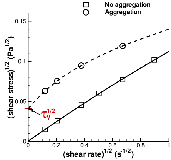
Figure 13: RBC aggregation and yield stress. A Casson plot with a polynomial fit showing the extrapolated intercept \tau_y for simulated suspensions with (dashed lines) and without (solid lines) aggregation at H_t = 0.45 . From Ref. [148].
