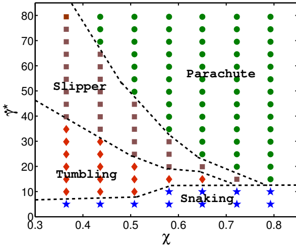
Figure 11: A phase diagram of RBC shapes in tube flow for Y_r = 18.9 \times 10^{-6} N/m , \kappa_r = 3 \times 10^{-19} J , which correspond to average membrane properties of a healthy RBC. Various dynamic states, depending on the flow strength characterized by \dot{\gamma}^* and the confinement \chi , are depicted by symbols: parachute (green circles), slipper (brown squares), tumbling (red diamonds) and snaking (blue stars) discocyte. The phase-boundary lines are drawn approximately to guide the eye. From Ref. [161].
