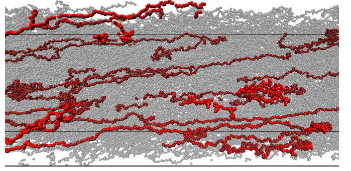
Figure 2: Snapshot of a systems with 800 polymers of length N_m = 250 for the Weissenberg number Wi_c = 184 . For illustration, some of the chains are highlighted in red. From Ref. [48].
