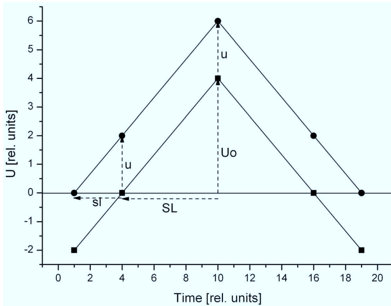
Figure 14. Sketch of zonal wind variation in summer (87.5 km; see text). Summer length is 2 \cdot SL . Increase of summer length is by 2 \cdot sl and results from an increase of zonal wind U by u .
