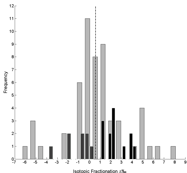
Fig. 3. Estimates of apparent fractionation associated with soil microbial respiration determined by different experimental approaches (grey bars: from C 3 plants; dark grey bars: Rayleigh distillation methods, black bars: C 4 plants). The dashed line is the mean of all estimates. Data sources: Werth and Kuzyakov, 2010; Wynn et al., 2005, 2006; Dietchon and Kellman, 2008.
