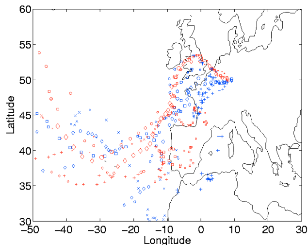
Fig. 15. Positions of FLEXPART clusters of trajectory particles initialized in 10-day backward simulations in CO layers observed on MOZAIC flights displayed on Fig. 14 (see text for details). Blue symbols are for 10 August 2003, 04:46:00 UTC flight, red ones are for 10 August 2003, 08:34:00 UTC flight). Over Portugal, clusters are 5 to 6 days old.
