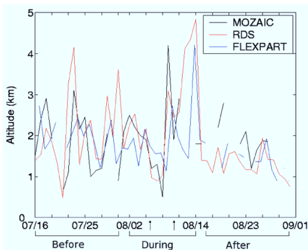
Fig. 5. Time series of planetary boundary layer height (km) as derived from MOZAIC profiles over Frankfurt (black), and radiosoundings at Idar-Oberstein, Stuttgart and Meiningen (red), and parameterized by FLEXPART for the grid cell covering Frankfurt (blue). MOZAIC profiles are selected between 09:30:00 UTC and 19:00:00 UTC. Radiosoundings are made at 12:00:00 UTC. Hours of FLEXPART diagnoses are those of MOZAIC flights.
