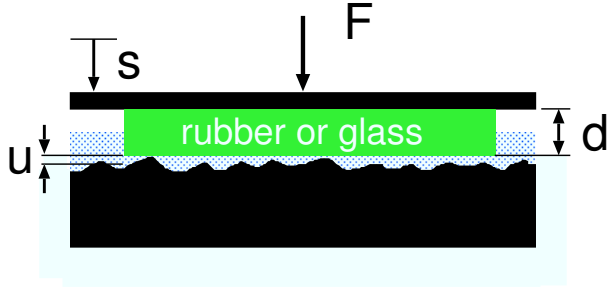
FIG. 6: Squeeze-out experimental set-up. A cylindrical glass or rubber block is squeezed against a substrate with a smooth or rough surface in a fluid. The cylindrical body has the height d = 0.5 cm thick and the diameter D = 2R = 3 cm. The normal load F_N = 13.8 N and the fluid viscosity \eta = 100 Pas. The vertical displacement u of the upper surface is registered as a function of time.
