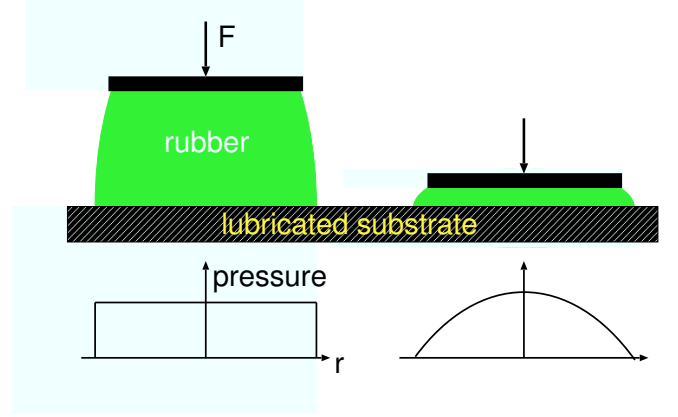
FIG. 3: A cylindrical rubber block (height d and radius R ) squeezed against a lubricated substrate (no friction). If d > R the pressure distribution at the interface will be nearly uniform (left) while if d \ll R (right) the pressure distribution will be nearly parabolic. We have assumed that the upper surfaces of the rubber cylinders are glued (no slip) to a flat rigid disk.
