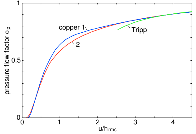
FIG. 2: The fluid pressure flow factor as a function of the average interfacial separation u divided by the root-mean-square roughness amplitude h_{\text{rms}} . For copper surfaces 1 and 2 . The green curve shows the large u -behavior predicted by Tripp[21].
