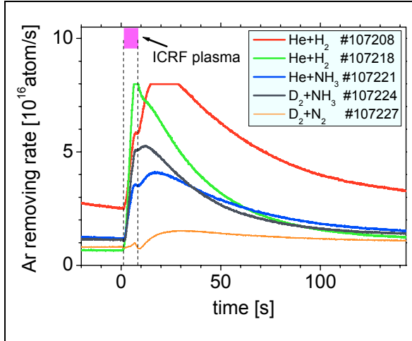
Fig 6: Ar removing rate for ICWC plasma application in different gas mixtures in TEXTOR. The TEXTOR walls were preloaded before each ICWC plasma with Ar in a GDC plasma in Ar/D_2
