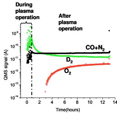
Fig 1: Residual QMS signal of mass 4 ( D_2 ), mass 28 ( CO+N_2 ) and M32 (mainly O_2 ) after plasma operation in TEXTOR under conditions with an air leak of about 2 \times 10^{-4} mbar/sec
