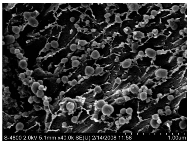
Fig. 6 Cryo-SEM micrograph of a mixture of TDMAO- \text{C}_6\text{F}_{13}\text{CO}_2\text{Li} with 50 mM, \alpha(\text{TDMAO}) = 0.5 and c(\text{HCl}) = 2.5 mM; mostly vesicles with a radius of 140 nm are formed.
