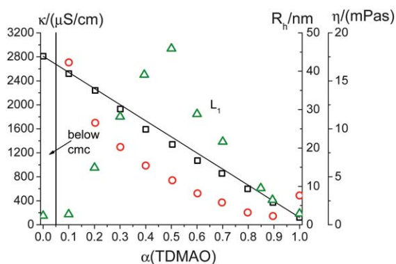
Fig. 2 TDMAO/ \text{C}_5\text{F}_{11}\text{CO}_2\text{Li} , 50 mM, T = 25^\circ\text{C} ; conductivity ( \kappa ) \square , hydrodynamic radius ( R_h ) \circ , and zero-shear viscosity ( \eta_0 ) \triangle .
