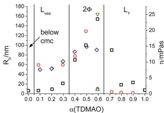
Fig. 4 TDMAO/ \text{C}_6\text{F}_{13}\text{CO}_2\text{Li} , 50 mM, T = 25 °C; viscosity ( \eta ) \square , hydrodynamic radius ( R_h ) determined with cumulant analysis \circ and for \alpha(\text{TDMAO}) = 0.6 with a bi-exponential fit of g^{(2)} \triangle and \nabla , and vesicle radius determined from the decrease of the conductivity \diamond .
