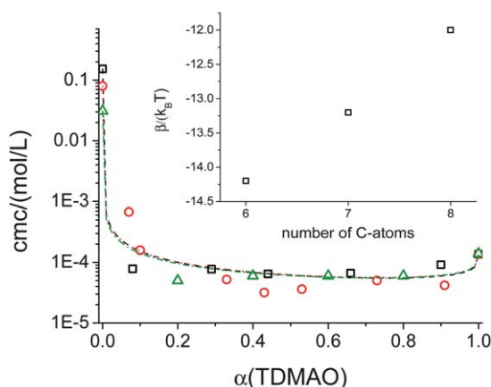
Fig. 1 Critical micelle concentration (cmc) determined by conductivity measurements; TDMAO-C 5 F 11 CO 2 Li measurement - □, theory with \beta = -14.2 - dashed line; TDMAO-C 6 F 13 CO 2 Li measurement - ○, theory with \beta = -13.2 - dotted line; TDMAO-C 7 F 15 CO 2 Li 21 measurement - △, theory with \beta = -12 - dashed-dotted line; inset: average interaction parameter ( \beta ) for the synergistic interaction between TDMAO and perfluoro carboxylates as a function of the length of the anionic perfluoro surfactant.
