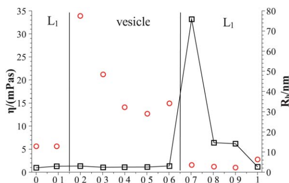
Fig. 7 TDMAO/ \text{C}_7\text{F}_{15}\text{CO}_2\text{Li} , 50 mM, T = 25 °C; hydrodynamic radius ( R_h ) (○) and viscosity ( \eta ) (□).
