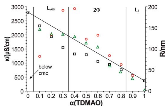
Fig. 3 TDMAO/HCl/ \text{C}_5\text{F}_{11}\text{CO}_2\text{Li} , 50 mM, T = 25^\circ\text{C} , (c(\text{HCl})/c(\text{TDMAO}) = 0.1) ; conductivity ( \kappa ) \square , and particle radius ( R ) determined by DLS measurements (hydrodynamic radius) \triangle and from the decrease of conductivity \circ .
