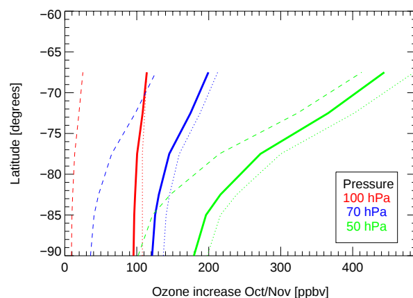
Fig. 7. As Fig. 6, but using an overhead ozone profile reduced by a factor of 5 between 30 and 150 hPa.
