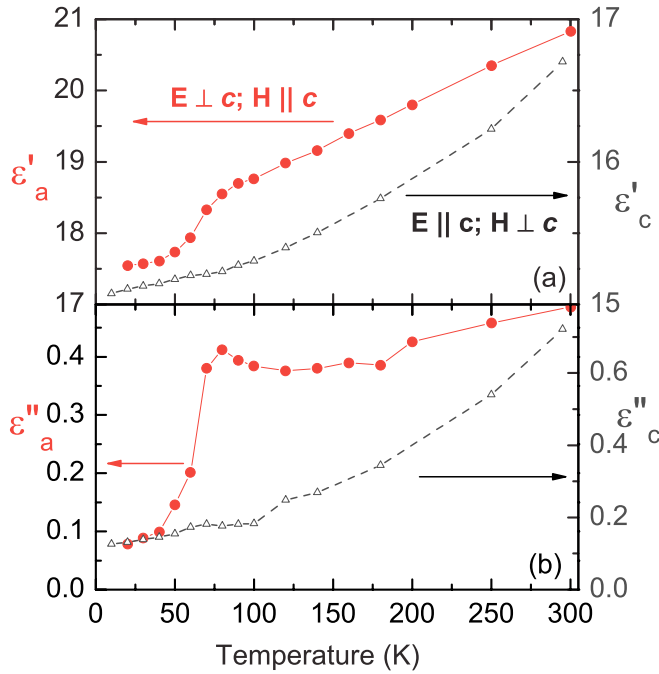
FIG. 6. (Color online) Temperature dependence of the (a) permittivity and (b) dielectric loss measured at 20 \text{ cm}^{-1} with polarization \mathbf{E} \perp \mathbf{c} (red solid lines) and \mathbf{E} \parallel \mathbf{c} (black dashed lines).
