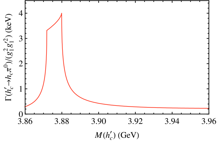
Figure 9: The width of the decay h'_c \rightarrow h_c \pi^0 considering only the meson loops.
