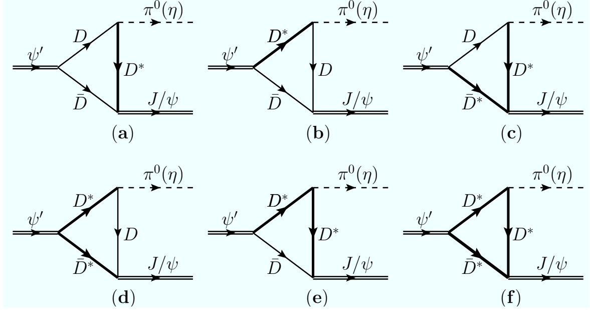
Figure 3: The decays \psi' \rightarrow J/\psi \pi^0(\eta) through triangle charmed-meson loops. Charmonia, light mesons, pseudoscalar and vector charmed mesons, are denoted by double, dashed, thin and thick solid lines, respectively.
