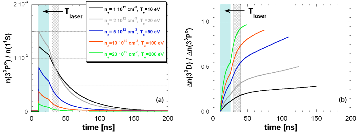
FIGURE 3. (a) Calculation of the relative fluorescence response at the laser wavelength as a result of a laser pulse at \lambda = 388.9 \text{ nm} performed for five different pairs of (n_e, T_e) . (b) Calculated ratio of the collisional- and laser-induced fluorescence signals upon the same laser pulse as in (a).
