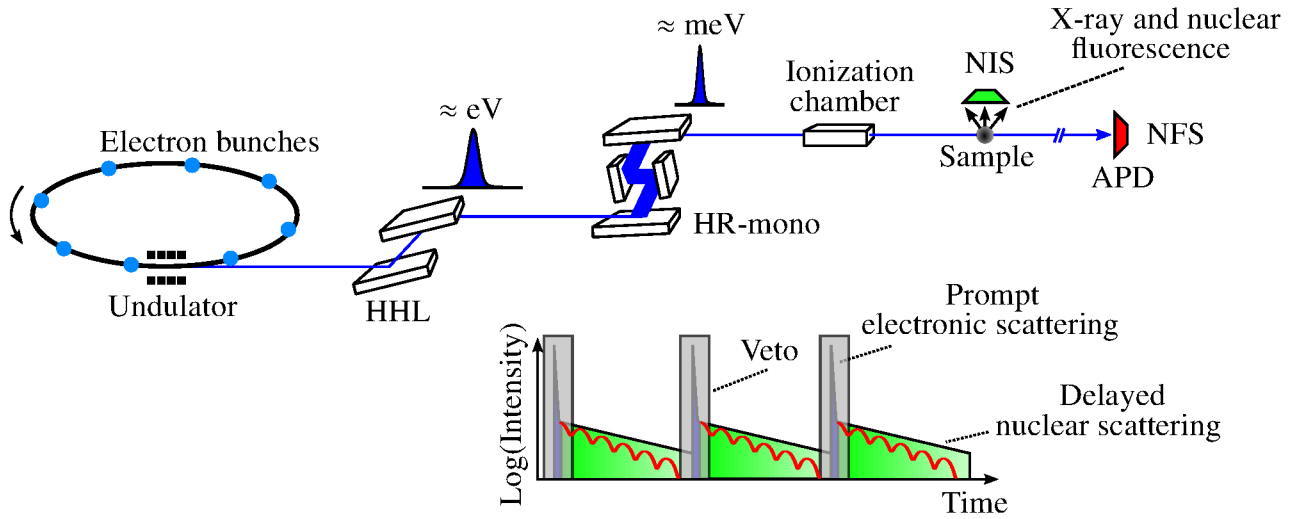
Figure 2.7: Basic setup of a nuclear resonance scattering beam line at a synchrotron. When the electron bunches pass through the undulator they emit synchrotron radiation which is subsequently monochromatized in two steps by a high heat load monochromator (HHL) to a few eV and by a high resolution monochromator (HR-mono) to a few meV. The intensity of radiation impinging on the sample is monitored using an ionization chamber. Silicon avalanche photodiode detectors (APD) are used to measure the nuclear forward scattering (NFS) and nuclear inelastic scattering (NIS) signal. The NIS signal is recorded by detecting the X-ray and nuclear fluorescence emitted by the sample after the decay of the excited Mössbauer nuclei via internal conversion. In both NFS and NIS the measured signal is analysed in time in order to separate the prompt electronic from the delayed nuclear scattering. Signals recorded in the first few ns after the synchrotron pulse are therefore rejected (Veto).
