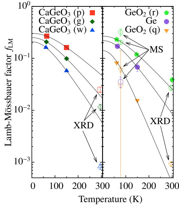
Figure 3.3: f_{\text{LM}}(T) (filled symbols) in \text{CaGeO}_3 garnet, perovskite and wollastonite, ^{73}\text{GeO}_2 quartz and rutile and ^{73}\text{Ge} obtained from the effective thickness \xi(T) . The lines are the fits according to the Debye approximation [14]. Open symbols correspond to Mössbauer spectroscopy (MS) [35, 36] and XRD results [49–53].
