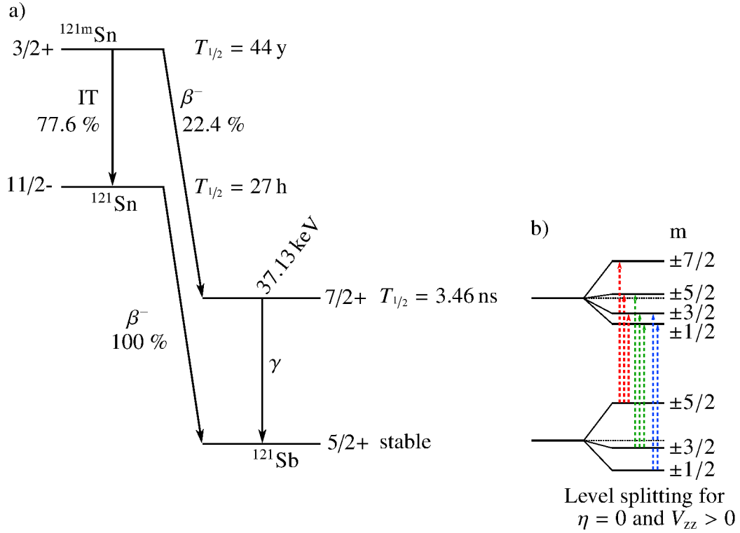
Figure 2.4: a) Decay scheme of ^{121\text{m}}\text{Sn} and the 7/2+ to 5/2+ Mössbauer transition of ^{121}\text{Sb} . Half lives, T_{1/2} , and branching ratios of internal conversion (IT) and \beta^- decay are given in the figure. Values are taken from Ref. [20]. b) Level splitting of the 5/2+ and 7/2+ states with respect to the magnetic quantum number, m , due to electric quadrupole interaction in case of an asymmetry parameter, \eta = 0 , and a positive electric field gradient, V_{zz} . The eight transitions allowed by the selection rules for a M1 transition, \Delta m = 0, \pm 1 , are also shown.
