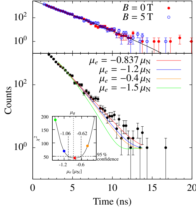
Figure 3.4: Top: NFS for \text{CaGeO}_3 wollastonite at 150 K with and without an applied magnetic field of 5 T. Lines are the fits to the data, with Eq. 3.4.1 and \xi = 0.41(4) . The two fits are not distinguishable. Bottom: NFS measured in \text{CaGeO}_3 wollastonite at 5 T and 150 K. The lines are modelled with different nuclear magnetic moments \mu_e of the excited state. Inset: The goodness of the fit criterion \chi^2 as a function of the nuclear magnetic moment \mu_e of the excited state.
