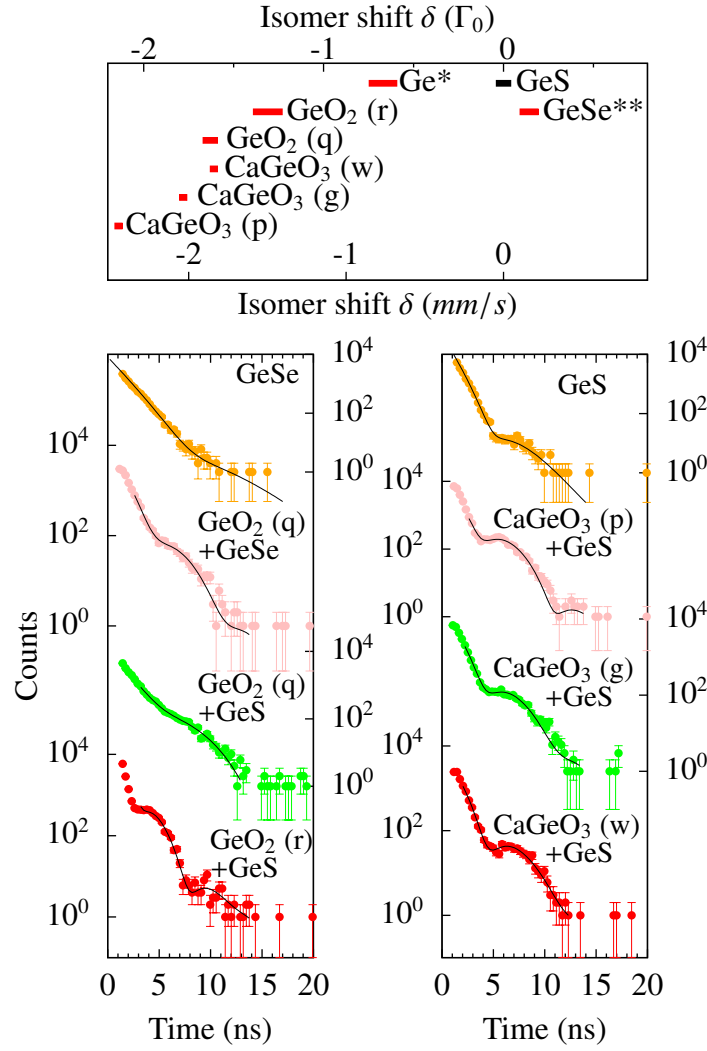
Figure 3.5: Left: The NFS of mixtures of ^{73}\text{GeO}_2 quartz and rutile with \text{GeS} at 98 and 298 K, respectively, of ^{73}\text{GeO}_2 quartz and \text{GeSe} at 15 K and of pure \text{GeS} and \text{GeSe} at 3 K. Right: The NFS of mixtures of the \text{CaGeO}_3 phases with \text{GeS} at 15 K. Lines are the fit to the data. Top: The isomer shifts with respect to \text{GeS} at 15 K. * \text{Ge} was calculated from our results and [35], [36]; ** \text{GeSe} from the \text{GeO}_2 vs. \text{GeSe} measurement.
