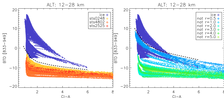
Fig. 21. Threshold functions (dashed line) for ice/STS (left) and ice/NAT (right) differentiation based on CSDB spectra in the altitude range 12–28 km for CI_A versus BTBD of the mean radiances of 832.3 to 834.4 \text{cm}^{-1} and 947.5 to 950.5 \text{cm}^{-1} . Dependency on STS composition (e.g. 0248 stands for 2 % \text{HNO}_3 and 48 % \text{H}_2\text{SO}_4 in orange to red) and radius (0.5 to 5 \mu\text{m} in green to light blue) are colour coded, respectively.
