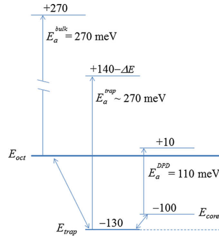
FIG 4 (color online). Ab initio results of site and activation energies (in meV) for hydrogen diffusion in the near partial dislocation core environment in Pd, relative to the bulk octahedral interstitial site, E_{\text{oct}} = 0 . \Delta E accounts for the slight reduction of the O-T trapping network, as discussed in the text. Vertical arrows indicate diffusion activation energy barriers. The site in the partial core is meta-stable with respect to the preferred trap site that resides just below the partial dislocation [33]. Solute hopping along core sites is associated with DPD, and core sites can only be accessed via the preferred trap sites.
