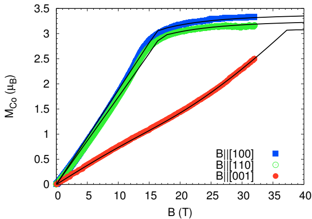
FIG. 5. (Color online) Magnetization of \text{Ba}_2\text{CoGe}_2\text{O}_7 with fields applied along [100], [110] and [001] directions (symbols from top to bottom respectively). Solid lines are results of calculations described in the text with parameters indicated in the text.
