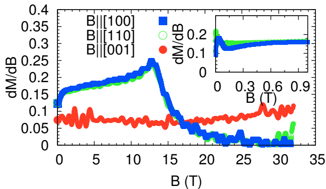
FIG. 6. (Color online) Field derivatives of magnetization, dM/dH , of \text{Ba}_2\text{CoGe}_2\text{O}_7 with fields applied along [100], [110] and [001] directions (symbols from top to bottom respectively). Inset shows the low-field region below 1 T.
