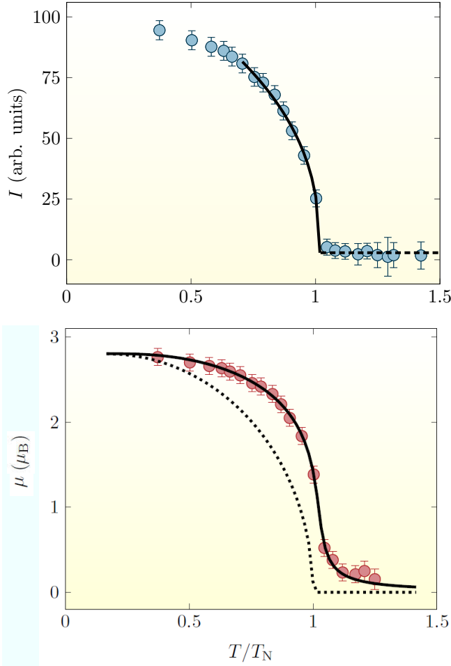
FIG. 4. (Color online) Upper panel: Temperature dependence of the integrated intensity of the magnetic (110) Bragg reflection. The experimental data (shown by circles) is taken by unpolarised single-crystal neutron diffraction. Solid line shows a fit to Eq. 5. The dashed line represents the nuclear (structural) contribution. Lower panel: Temperature dependence of the Co magnetic moment for \text{Ba}_2\text{CoGe}_2\text{O}_7 . The experimental data from the single-crystal neutron diffraction measurements are shown by circles. The solid line is a result of a modified molecular field model (Eq. 7). The dotted line is shown to illustrate the deviation of \mu(T) from the conventional molecular field model (Eq. 6).
