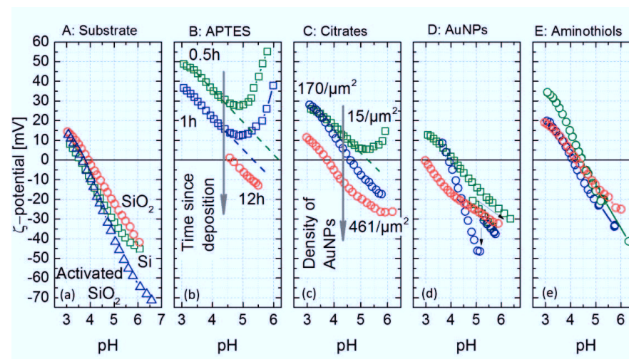
Figure 44: pH dependence of the \zeta potential of: (a) bare substrates Si, Si/SiO 2 and oxygen activated Si/SiO 2 , (b) after deposition of APTES (measured different time after APTES deposition), (c) after deposition of citrate-stabilized AuNPs (different AuNP concentrations are given), (d) after removal of free molecules (citrate and APTES) via oxygen plasma, and (e) after deposition of amino-1-undecanethiols onto the AuNPs. Each curve represents a different pair of samples, however, experiments in the same symbol (and color) belong to one series of measurements (e.g. identical density of AuNPs), and excluding step A, which is the same for all. Additional lines in (b) and (c) indicate the extrapolation of the measurement that is used to obtain an IEP value for some of the measurements.
