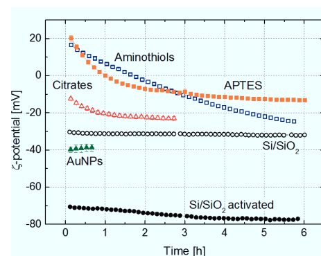
Figure 45: Time dependence of the \zeta potential of Si/SiO 2 substrate (open circles), Si/SiO 2 substrate, treated by oxygen plasma (solid circles), positively charged layer of APTES molecules (solid squares), positively charged layer of amino-1-undecanethiols pinned on the AuNPs (open squares), citrate-stabilized AuNPs on APTES possessing both negative charges from citrate-molecules on gold and positive charges from APTES (open triangles), and plasma-treated bare AuNPs on a bare substrate (solid triangles). All measurements were executed at pH of 6.
