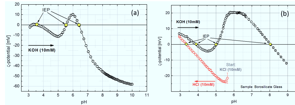
Figure 31: pH dependence of \zeta potential of borosilicate glass for "complete" titration without N_2 purger. In both cases the experiment starts at pH of \sim 5.5 with an acidic titration using HCl (3.2ml HCl (0.1M) in one step (a) and HCl (10mM) in reasonable number of steps in (b)), followed by a stepwise basic titration using KOH (10mM).
