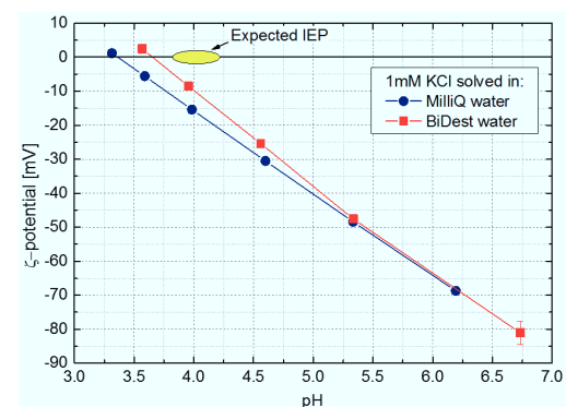
Figure 28: pH dependence of the \zeta -potential of polypropylene foil measured with 1mM KCl solved in MilliQ (blue circles) and double distilled water (BiDest) (red rectangles).
