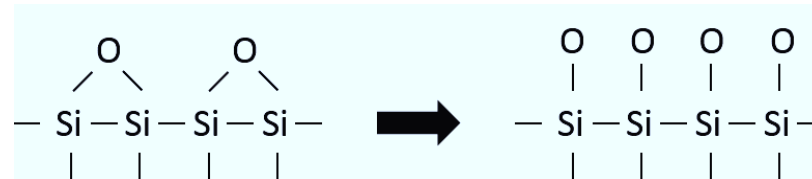
Figure 10: Silanol bonds reconstruction, due to e.g. activation via oxygen plasma. Adapted from [37].
