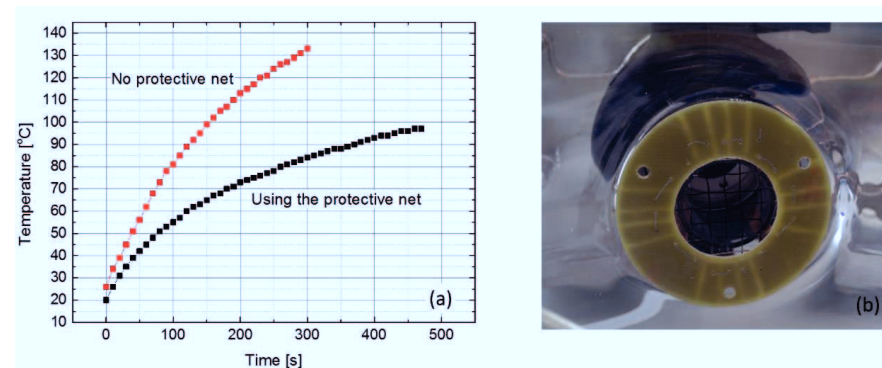
Figure 18: (a) Temperature rise inside the chamber with and without using the (b) protective net.
