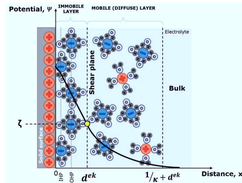
Figure 4: Schematic structure of the electrical double layer (EDL), according to the Gouy-Chapman-Stern-Grahame (GCSG) theory.
