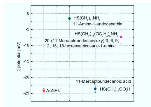
Figure 49: Comparison of the \zeta potential at a pH 7.2 (in HBSS as electrolyte) for an activated Si/SiO 2 substrate with AuNPs (step E) functionalized with different molecular monolayers: 11-mercaptoundecanoic acid (blue), 20-(11-mercaptoundecanyloxy)-3,6,9,12,15,18-hexaoxaicosane-1-amine (magenta), and 11-amino-1-undecanethiol (green). Additionally, the \zeta potential of the sample (Si/SiO 2 with AuNPs) without functionalization is given.
