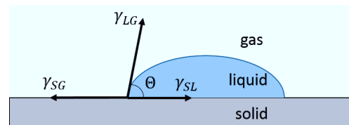
Figure 22: Contact angle \theta of three-phase solid/liquid/gas system with interfacial energies \gamma_{SL} , \gamma_{SG} , \gamma_{LG} of solid/liquid, solid/gas and liquid/gas interfaces respectively.
