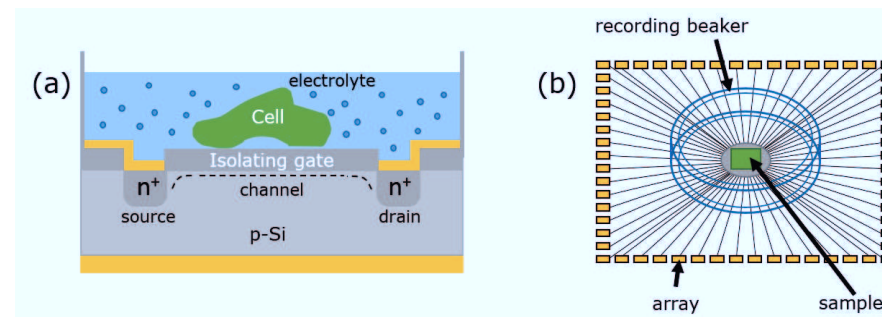
Figure 2: The schematic example of bioelectronic devices: a) ion-sensitive field effect transistor (ISFET) and b) multi-electrode array (MEA).
