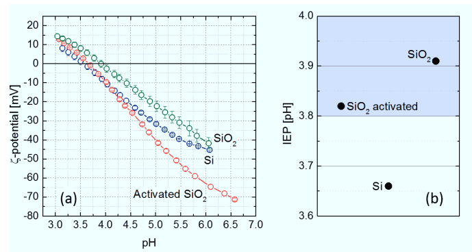
Figure 34: pH dependence of the \zeta potential of n-doped Si (100) after cleaning (blue circles), with additional 100nm SiO 2 layer (green circles) and additional oxygen activation (red circles). The shaded region in (b) marks the regime of hydrophobic inert surfaces.
