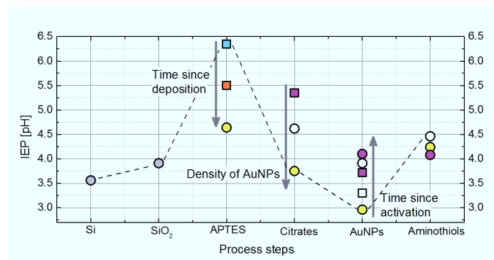
Figure 47: Resulting IEPs for the different process steps of immobilization and functionalization of gold nanoparticles, given in Figure 44. The dashed line shows the resulting modification of the \zeta potential. Different colors represent the different data sets.
