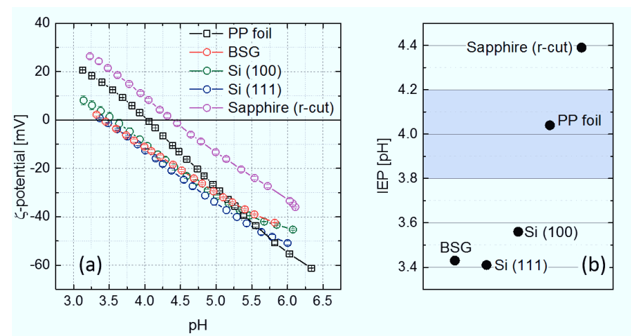
Figure 33: a) pH dependence of the \zeta potential and b) isoelectric points of 'simple' dielectric interfaces (i.e. borosilicate glass, silicon (111) and (100) orientation, r-cut sapphire) in comparison to the polypropylene foil. The shaded region in (b) marks the regime of hydrophobic inert surfaces.
