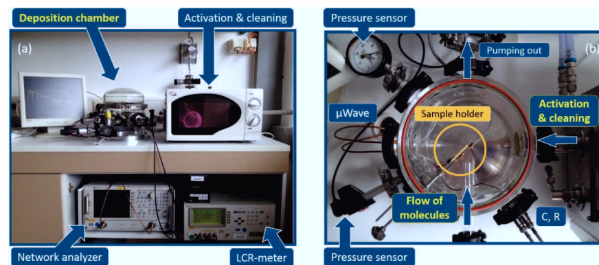
Figure 14: GLOBUS - The novel concept device for deposition of molecular monolayers, including in-situ cleaning and activation of substrates as well as in-situ electronic characterization of molecular monolayers: a) overview, b) top view.
