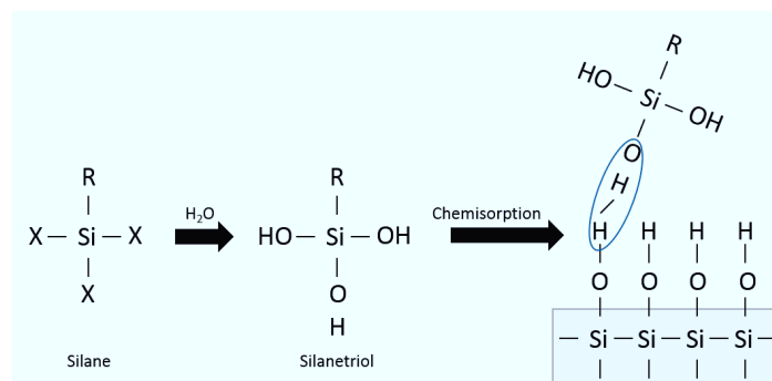
Figure 12: Silanization mechanism presented schematically.
