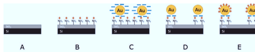
Figure 20: The schematic description of the process steps, i.e. A: Si and Si/SiO 2 substrate, B: substrate functionalized with APTES, C: immobilization of citrate-stabilized AuNPs, D: removal of free citrates and APTES ligands, and E: decoration of AuNPs with aminothiols. For details, see text.
