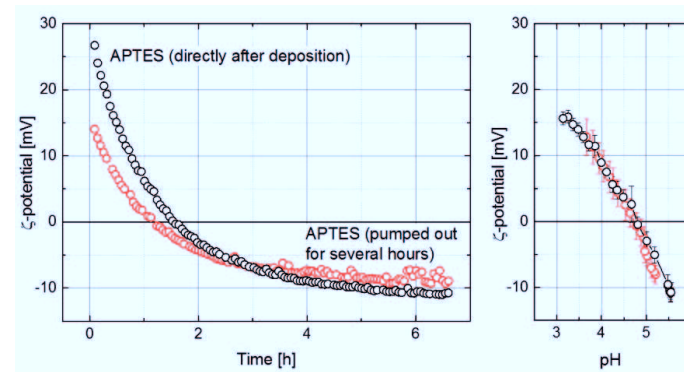
Figure 46: (a) Time dependence (measured at a pH of 6) and (b) pH dependence of the \zeta potential of APTES monolayers on Si(100).
