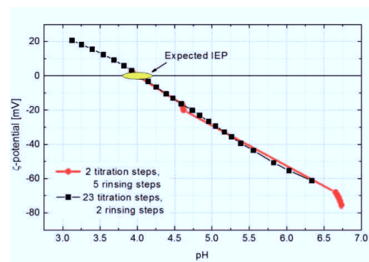
Figure 29: \zeta potential as a function of pH of a PP foil for improved measurement procedures using BiDest water, N_2 purger and sufficiently long rinsing pauses in between titration steps.
