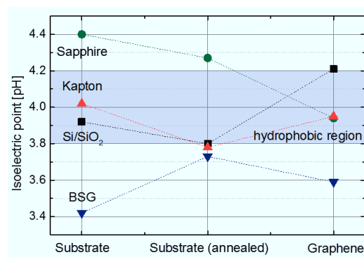
Figure 39: Comparison of IEPs for graphene layers on different substrates, original substrates and N 2 annealed substrates. Lines are guides for the eyes. The shaded regime represents the regime of IEP for hydrophobic materials.
