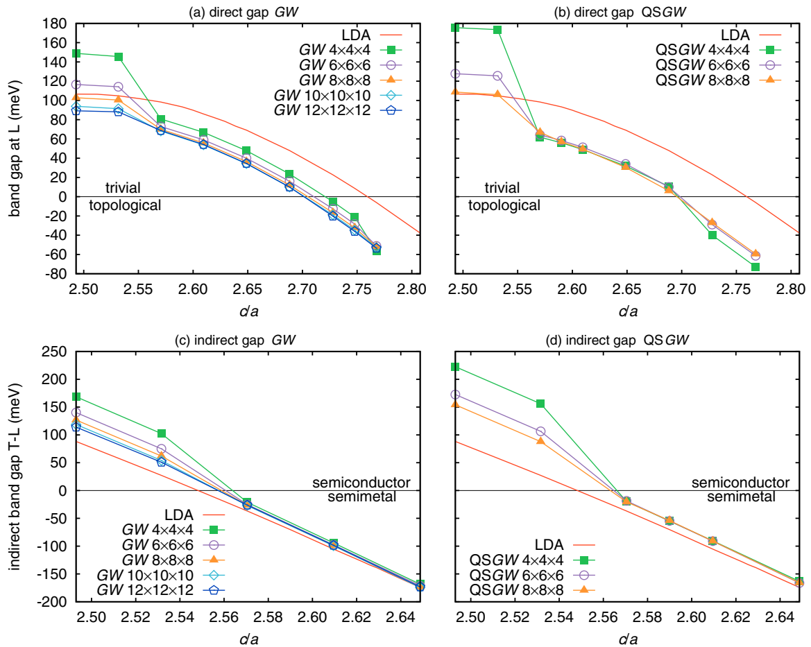
FIG. 5. (Color online) LDA, GW , and QSGW values of the direct and indirect band gaps of bulk Bi as a function of the ratio c/a for different \mathbf{k} -point sets, but for a set of reduced convergence parameters; see text.
