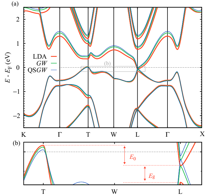
FIG. 2. (Color online) LDA, GW , and QSGW band structures of bulk Bi. The inset in (b) shows the electron and hole pockets together with the E_g and E_0 gaps corresponding to the LDA bands.
