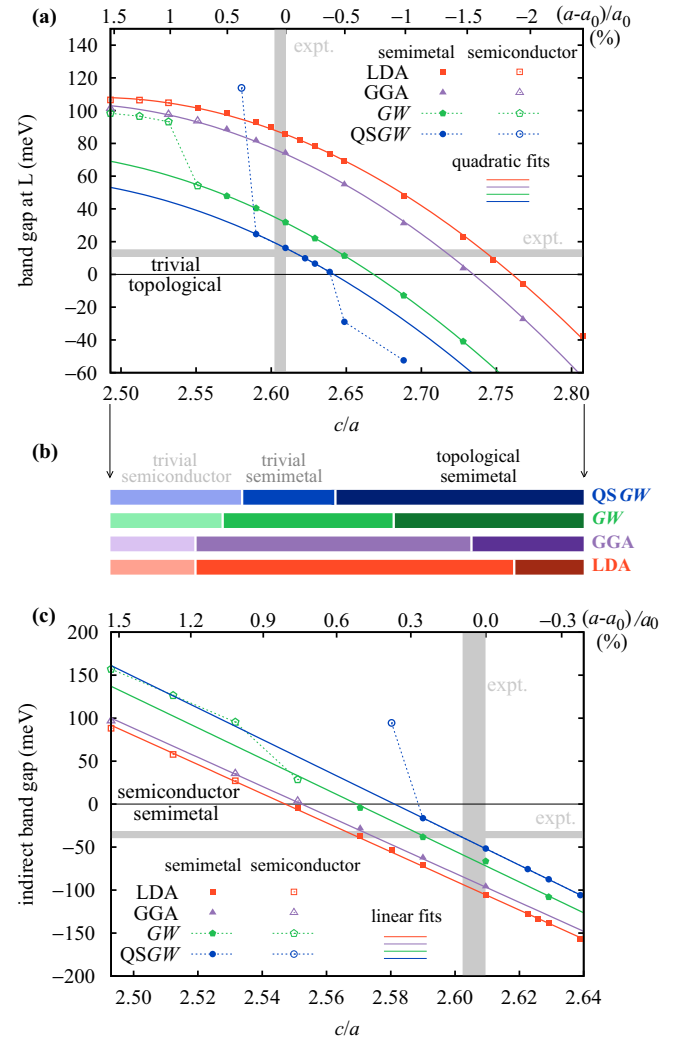
FIG. 3. (Color online) (a) LDA, GGA, GW , and QSGW direct band gap E_g of bismuth at L for different strains (varying the ratio c/a and keeping the volume constant). (b) Three electronic phases are found for Bi as a function of the ratio c/a within all the approaches. (c) LDA, GGA, GW , and QSGW indirect band gap E_0 of bismuth for different values of c/a . On the upper x axis of (a) and (c), we show the percentage of in-plane strain. The range of experimental values of c/a [31], the experimental gap at L [11–15], as well as the experimental indirect gap [13,15,29,30] are represented as gray shaded areas in (a) and (c). Small differences to the QSGW values in Table I are due to the use of a reduced \mathbf{k} -point set; see Appendix.
