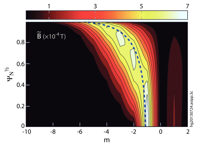
FIG. 5. Contour plot of the magnetic perturbation spectrum showing the Fourier amplitude of the radial component of the toroidal n = 1 magnetic field for the H-mode discharge shown in Fig. 4 with q_{95} = 3.8 , calculated with a total helical filament current of 1.5 kA, uniformly distributed across the current filaments induced by LHCD in the boundary plasma. \psi_N is the normalized poloidal magnetic flux and m is the poloidal mode number. The pitch resonant modes with m = nq(\psi) are shown by the dashed line.
