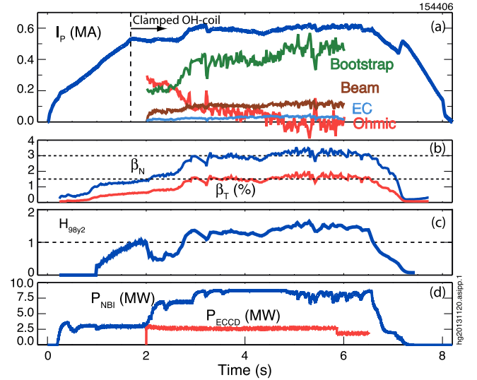
FIG. 15. Demonstration of a fully noninductive H-mode plasma achieved in DIII-D with plasma parameters and plasma formation consistent with capabilities expected for EAST in 2014.
