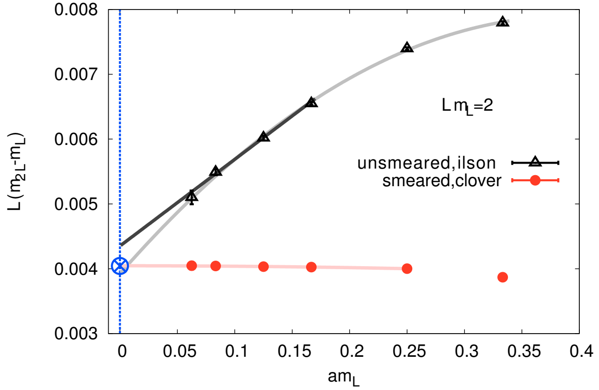
Figure S4: Continuum scaling of a mass difference in QED_L using two different lattice actions. The crossed circle in the continuum limit is the analytical result from the expressions of Sec. 3 (see text). The fitted curves are described in the text.
