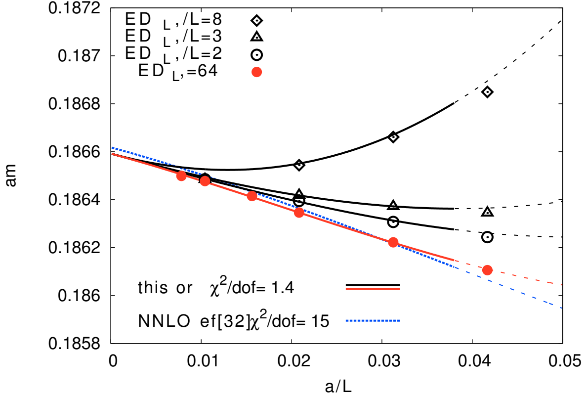
Figure S3: Finite-size dependence of the fermion mass in two different realizations of finite-volume QED, that differ in the zero-mode subtraction. The open/filled symbols are obtained using QED_{TL}/QED_L prescription. The curves are the analytical formulae from Eqs. (S22) and (S24). The dotted curve is the NNLO formula from Ref. (32).
