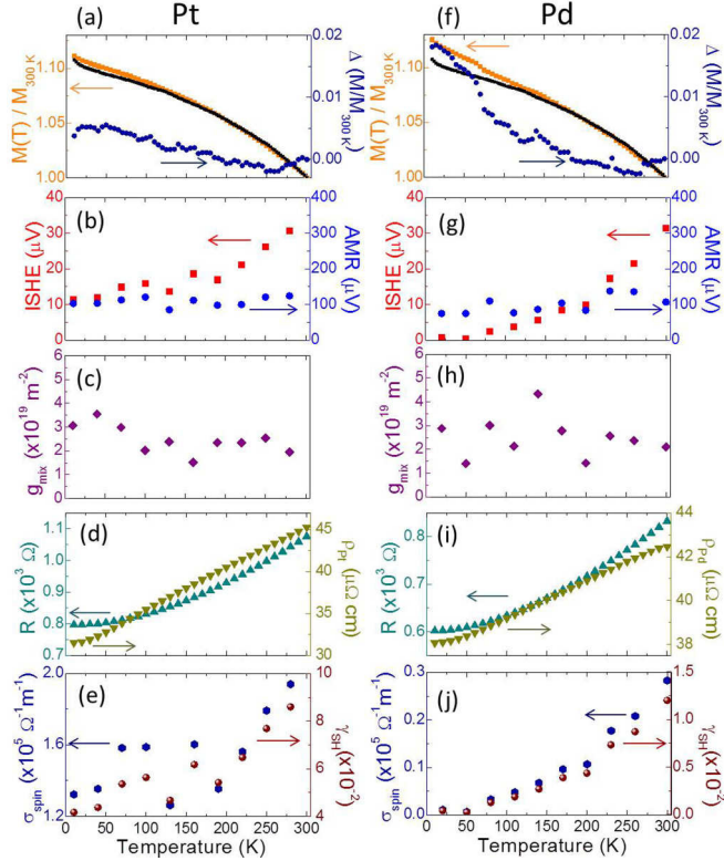
FIG. 5. (Color online) Temperature dependence of (a) normalized magnetization, M(T)/M_{300K} (with respect to 300 K) of Py/Pt and Py and their differences ( \Delta ), measured by a SQUID magnetometry with 2k Oe in-plane applied field. (b) AMR and ISHE voltage amplitudes at 4 GHz, (c) spin mixing conductance, (d) device total resistance and Pt resistivity, and (e) calculated spin-Hall angle and spin-Hall conductivity for Pt. Right panels (f)–(j) are corresponding results for Pd.
