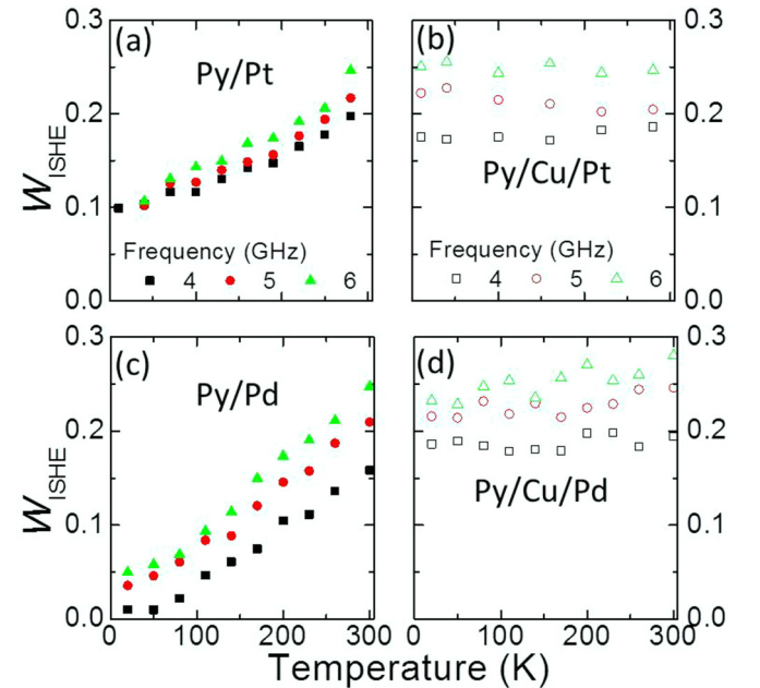
FIG. 4. (Color online) Temperature dependence of W_{\text{ISHE}} at 4, 5, and 6 GHz for (a) Py/Pt, (b) Py/Cu/Pt, (c) Py/Pd, and (d) Py/Cu/Pd bilayers.
