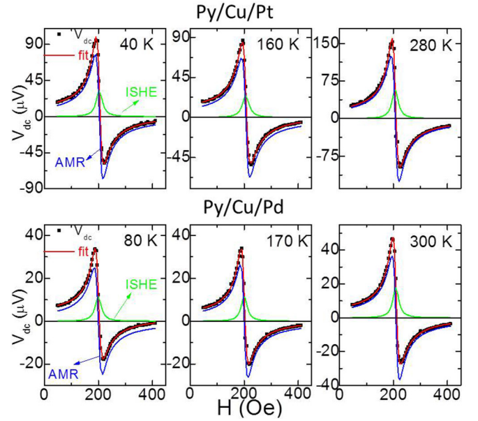
FIG. 3. (Color online) DC voltage spectra measured at 4 GHz for Py/Cu/Pt and Py/Cu/Pd reference samples at selective temperatures.
