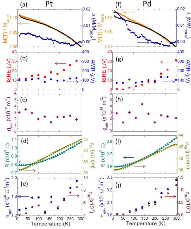
FIG. 5. (Color online) Temperature dependence of (a) normalized magnetization, M(T)/M_{300K} (with respect to 300 K) of Py/Pt and Py and their differences ( \Delta ), measured by a SQUID magnetometry with 2k Oe in-plane applied field. (b) AMR and ISHE voltage amplitudes at 4 GHz, (c) spin mixing conductance, (d) device total resistance and Pt resistivity, and (e) calculated spin-Hall angle and spin-Hall conductivity for Pt. Right panels (f)–(j) are corresponding results for Pd.
