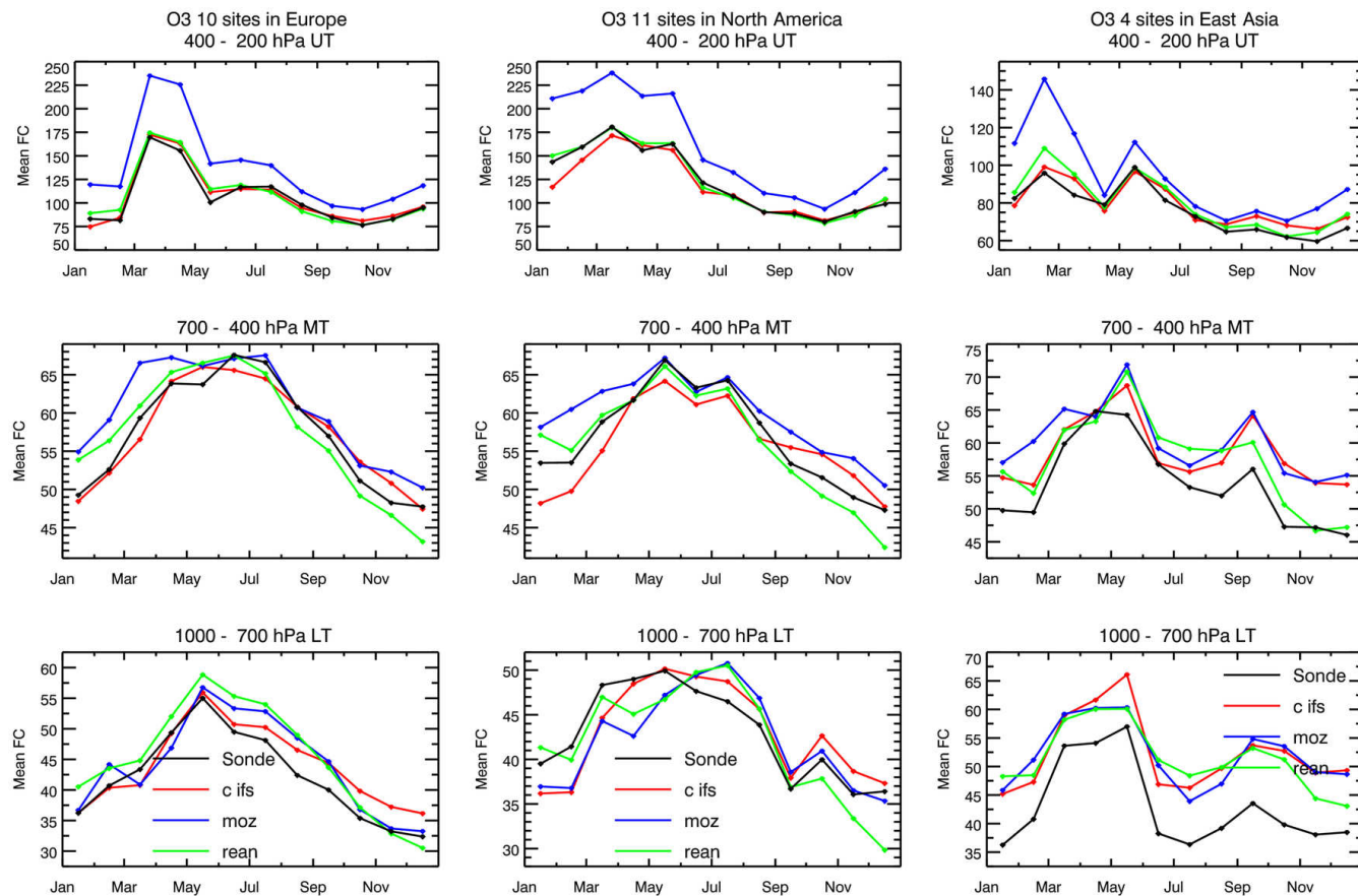
Figure 2. Tropospheric ozone volume mixing ratios (ppb) over Europe (left) and North America (middle) and East Asia (right) averaged in the pressure ranges 1000–700 hPa (bottom), 700–400 hPa (middle) and 400–200 hPa (top) observed by ozonesondes (black) and simulated by C-IFS (red), MOZ (blue) and REAN (green) in 2008.
