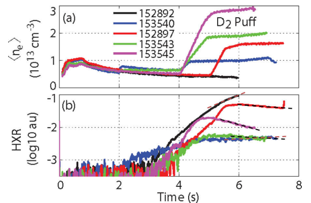
FIG. 9. DIII-D measurements of density and log(HXR) on 5 shots are shown, with linear fits (dashed lines) to determine growth and decay rates. Low densities early in the discharges promote RE growth. Densities are increased later in the discharges to suppress the runaways. (Adapted with permission from Ref. 6; copyright 2014 American Institute of Physics.)
