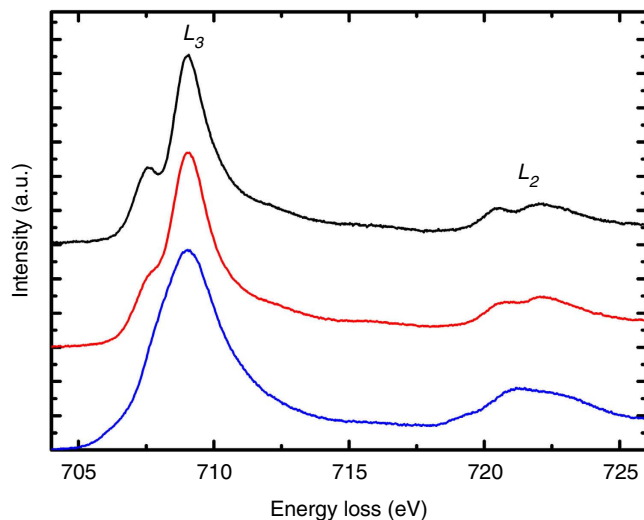
Figure 2 | EEL spectra acquired from reference iron oxide samples. EELS analysis of the Fe 2p L_{2,3} edge experimentally acquired from pure samples of \text{Fe}_3\text{O}_4 (blue), \gamma\text{-Fe}_2\text{O}_3 (red) and \alpha\text{-Fe}_2\text{O}_3 (black).
