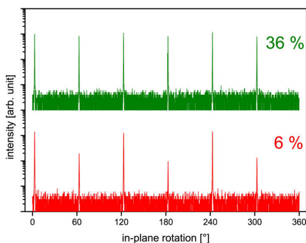
Figure 8. Pole scans of the \{015\} reflections of 100 nm \text{Bi}_2\text{Se}_3 for growth on rough (red) and flat (green) \text{InP}(111)\text{A} substrates. The twin volume on A-type substrates (indicated) also demonstrates twin suppression on rough substrates.
