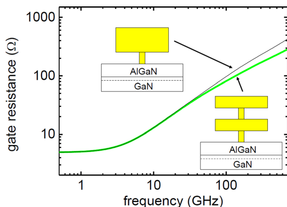
FIG. 2. Calculated gate resistance as function of frequency for T-gate vs. DLTG structure.
