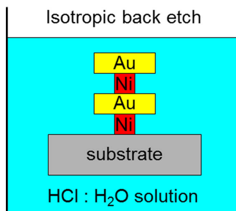
FIG. 4. Schematics of wet etching process for double-level-T-gate fabrication.
