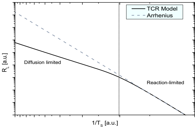
Fig. 4. Arrhenius plot, showing the transition from reaction (low temperature T_s , right part) to diffusion (high T_s , left part) limitation of thermo-chemical removal (TCR) with temperature (dotted line) and the resulting decrease of the removal rate R_L below the Arrhenius behaviour (dashed line), which is the expectation without reaction partner density effects.
