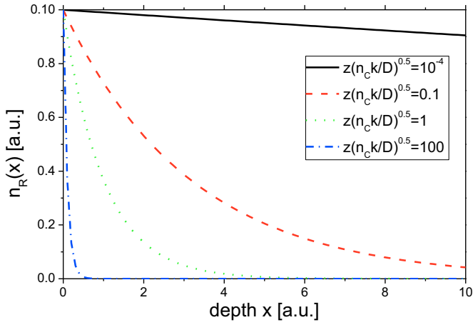
Fig. 3. Parameter study showing the effect of z\sqrt{n_c k/D} on the reactive gas concentration in depth x . The local removal rate is proportional to the local reactive gas concentration (Eq. (6)).
