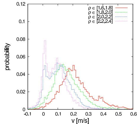
Figure 1.6: Experimental velocity distribution [25].
