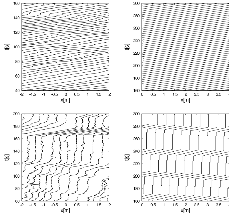
Figure 5.4: Experimental (top left) and model (top right) trajectories for N = 45 , \rho = 1.73 \text{ m}^{-1} . Experimental trajectories for N = 70 , \rho = 2.7 \text{ m}^{-1} (bottom left), and model trajectories for N = 65 , \rho = 2.5 \text{ m}^{-1} (bottom right).
