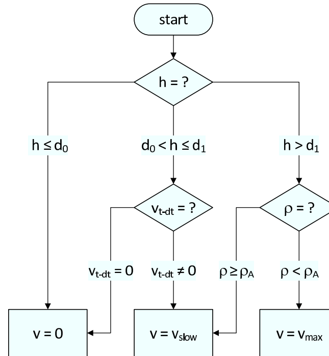
Figure 4.16: Schematic view of the algorithm calculating the new velocity of an updating agent. v_{t-dt} denotes v_i(d - dt) ; the index i has generally been omitted for better readability.
