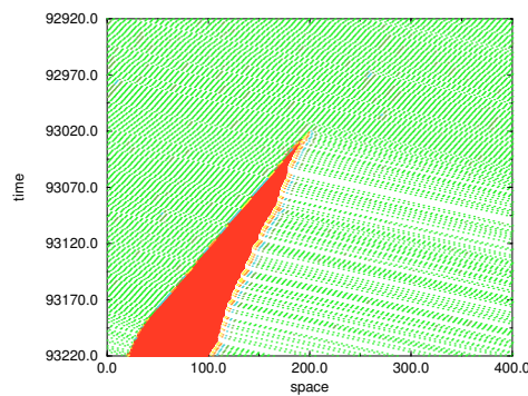
Figure 4.2: Simulated car trajectories in the VDR model [86].
