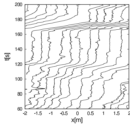
Figure 4.1: Experimental trajectories featuring phase separation.
