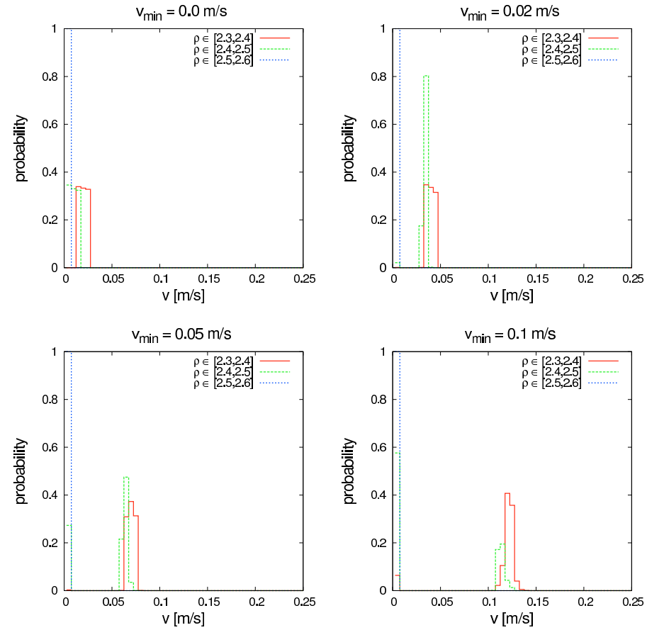
Figure 5.25: Model velocity distributions for different minimum velocities.
