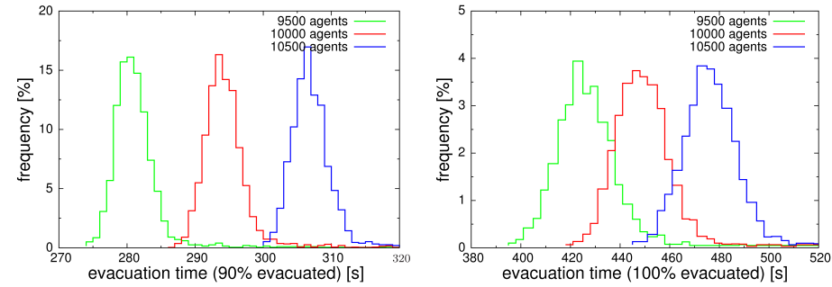
Figure 3.13: Distribution of evacuation times.
