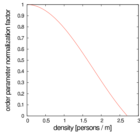
Figure 5.11: Normalization factor for the order parameter.
