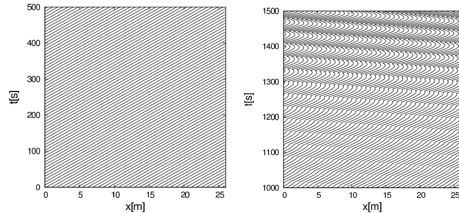
Figure 4.7: GCFM trajectories using the almost homogeneous initial condition at different stages of the simulation. Only every second agent is drawn to avoid cluttering up the plot. Data courtesy of Mohcine Chraïbi.
