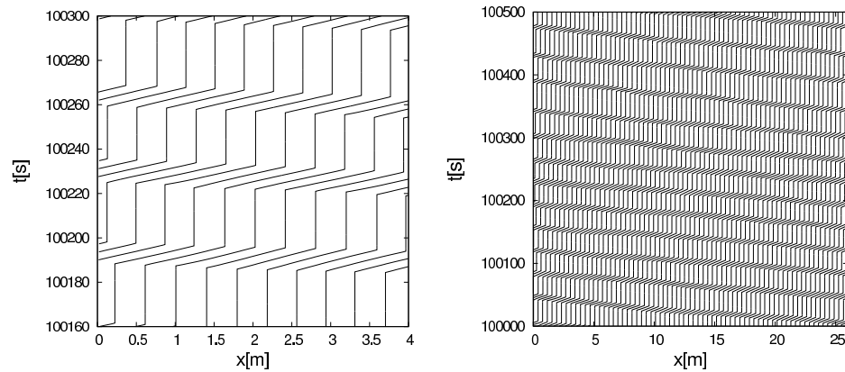
Figure 5.7: Zoomed-in (left) and global (right) trajectories for N = 65 , \rho = 2.5 \text{ m}^{-1} , after a long simulation time.
