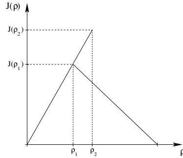
Figure 4.3: Schematic fundamental diagram of the VDR model [53].
