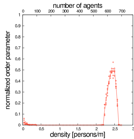
Figure 5.28: Order parameter at system size L = 260 m.
