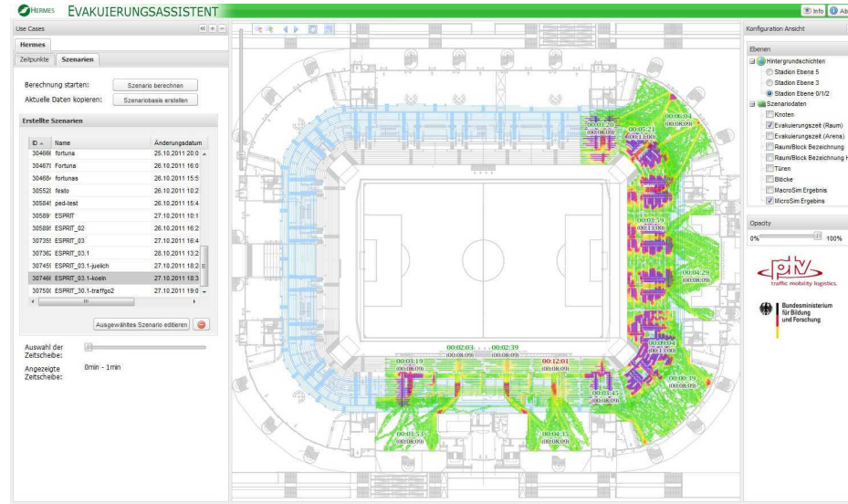
Figure 3.3: User interface of the evacuation assistant.
