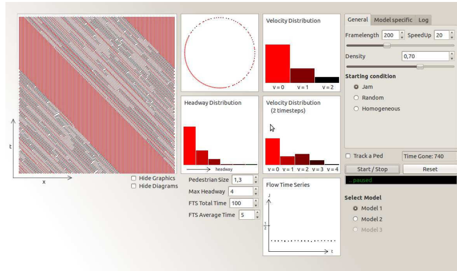
Figure 4.12: Screenshot of the simulation GUI.
