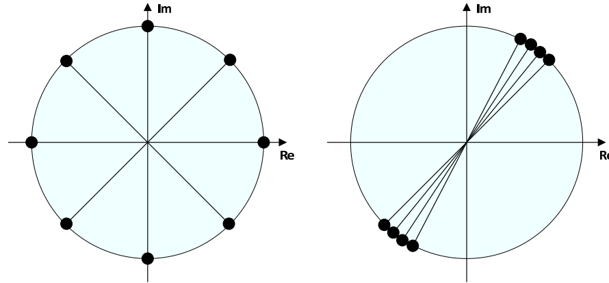
Figure 5.9: Homogeneous distribution of agents (left), two opposing jams (right).
