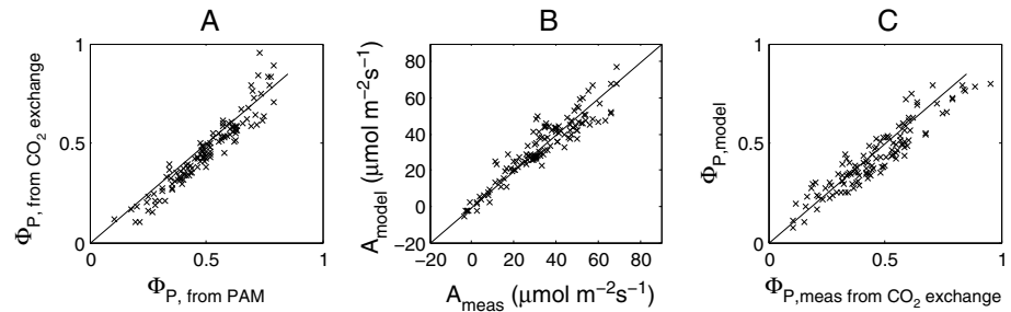
Figure 2. Cotton data of (a) photochemical yield \Phi_p from gas exchange versus \Phi_p from PAM, (b) modeled [Collatz et al. , 1991] versus measured photosynthesis, and (c) modeled versus measured (from gas exchange) \Phi_p .
