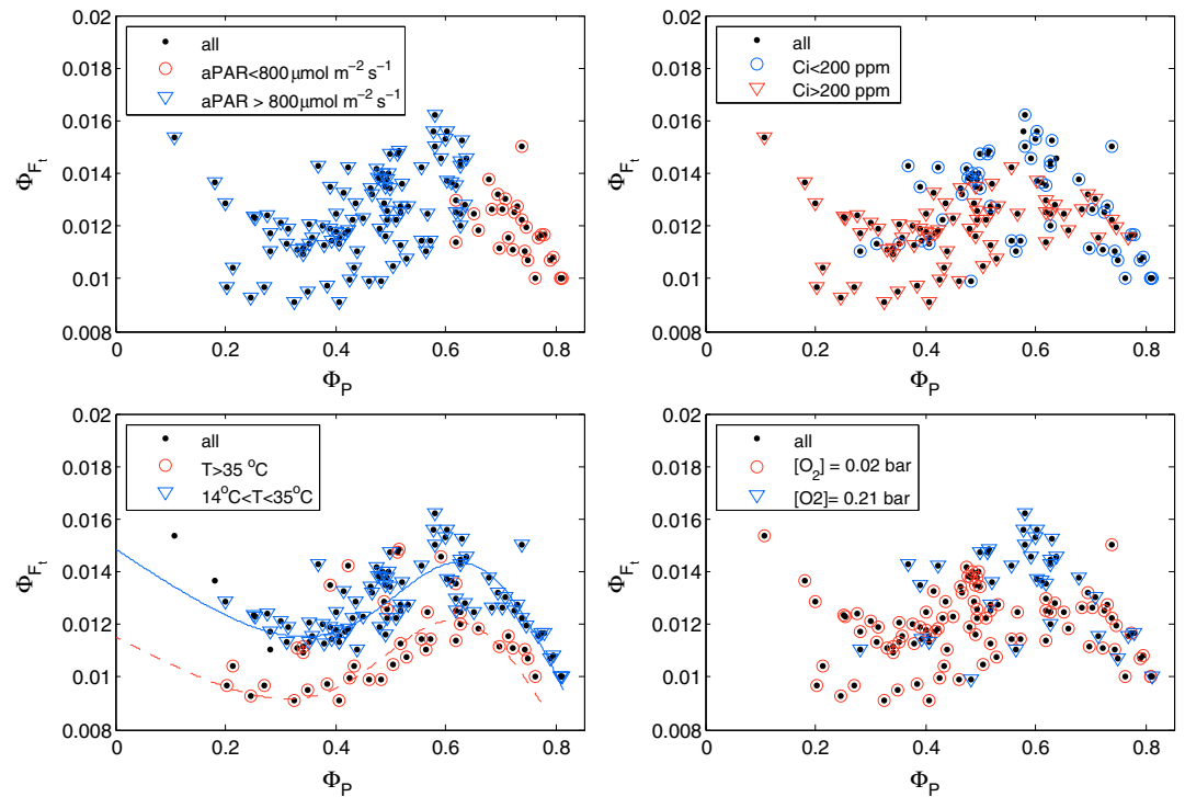
Figure 3. The data and model results of the cotton experiment presented as \Phi_{F'} versus \Phi_P , with different symbols for driving variables. The lines are computed from the empirical K_N(x) with temperature correction for 25°C (solid line) and 35°C (dashed line).
