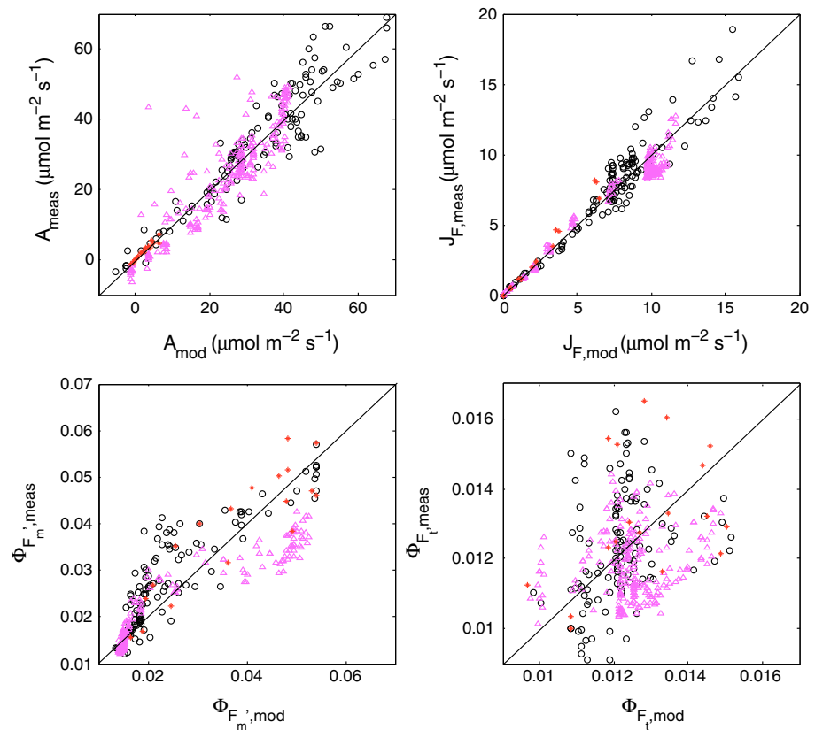
Figure 8. Modeled versus measured photosynthesis A , fluorescence flux ( \Phi_{F_t} \cdot d\text{PAR} ), steady state fluorescence yield \Phi_{F_t} , and maximum fluorescence yield \Phi_{F_m} (clockwise). Circles refer to cotton, triangles to maize, and stars to tobacco.
