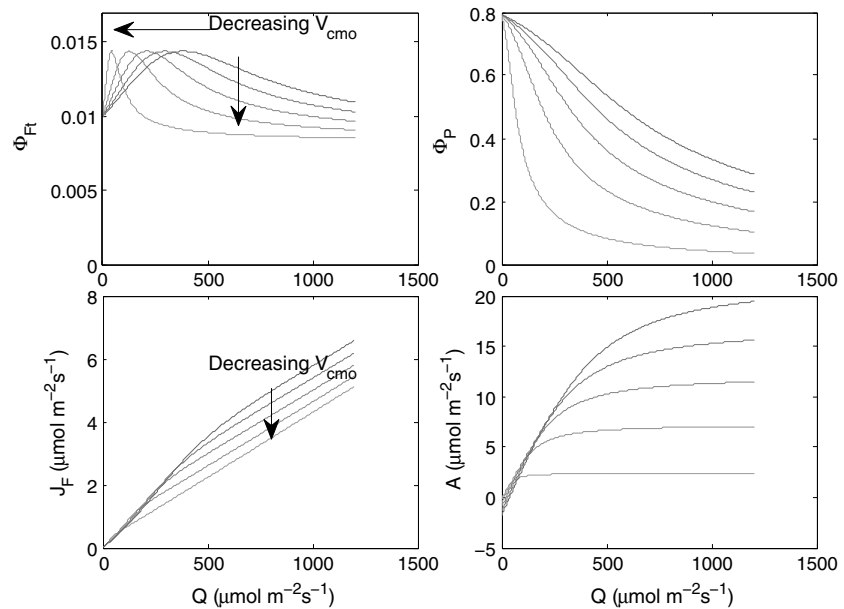
Figure 12. (top left) Modeled fluorescence yield \Phi_{Ft} (top right) photochemical yield \Phi_P , (bottom left) photosynthesis A , and (bottom right) fluorescence flux J_F , as functions of irradiance for the following values of maximum carboxylation capacity V_{\text{cmo}} : 10 (light gray), 30, 50, 70, and 90 (black) \mu\text{mol m}^{-2} \text{s}^{-1} . The drought relation between x and K_N was used.
