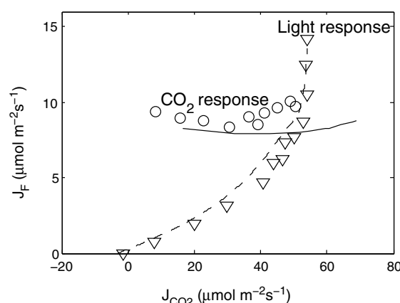
Figure 10. Selection of the cotton data for one light response curve (triangles) and one \text{CO}_2 response curve at an incident PAR of 1400 \mu\text{mol m}^{-2} \text{s}^{-1} (circles), with \text{CO}_2 gas exchange flux on the horizontal axis and fluorescence flux J_F = \Phi_F \cdot a\text{PAR}/2 from PAM data on the vertical axis. The lines are model results (cotton parameters for K_N(x) ) after coupling the PAM fluorescence model to the model of Collatz et al. [1991].
