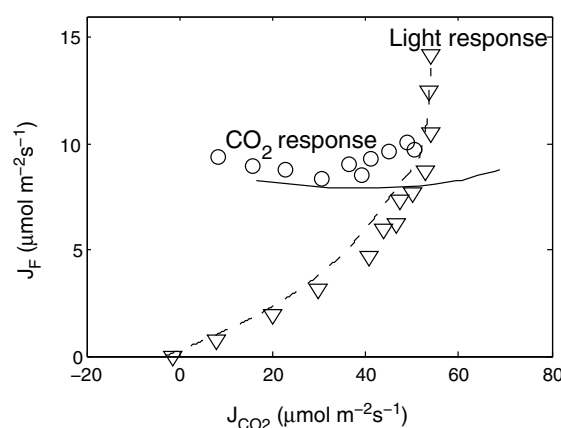
Figure 10. Selection of the cotton data for one light response curve (triangles) and one CO 2 response curve at an incident PAR of 1400 μmol m -2 s -1 (circles), with CO 2 gas exchange flux on the horizontal axis and fluorescence flux J_F = \Phi_F \cdot aPAR/2 from PAM data on the vertical axis. The lines are model results (cotton parameters for K_N(x) ) after coupling the PAM fluorescence model to the model of Collatz et al. [1991].
