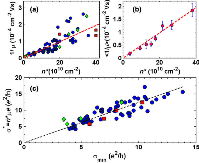
FIG. 3. (a) Same data as those of Fig. 2(c) plotted as 1/\mu - n^* , showing an overall linear relation. (b) Average inverse mobility as function of n^* (obtained as indicated in the main text), showing clearly the linearity of the relation. In (a) and (b) the dashed lines are a linear fit to the data, (1/\mu) = (h/e)n^* \times 0.118 . (c) minimum conductivity \sigma^* = n^*e\mu , calculated from the estimated carrier density fluctuations n^* and mobility \mu , and plotted as a function of measured minimum conductivity. The excellent overall agreement (the dashed line has slope 1) confirms the correctness of the procedures used to extract n^* and \mu from the measurements.
