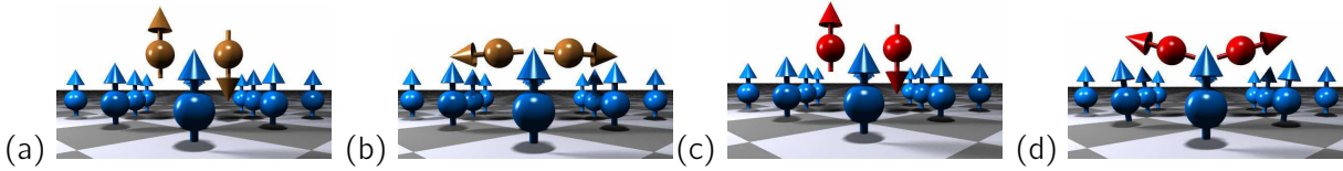
FIG. 6: Most stable configurations of Cr/Mn dimer obtained with (a/c) the collinear KKR method and (b/c) the non-collinear KKR method. The rotation angle with respect to the z axis is equal to 94.2^\circ/72.6^\circ . While the non-collinear state is the ground state for Mn-dimer it is only a local minimum for Cr-dimer. Atoms in blue correspond to the Ni substrate. Adapted with permission from Ref.[39].
