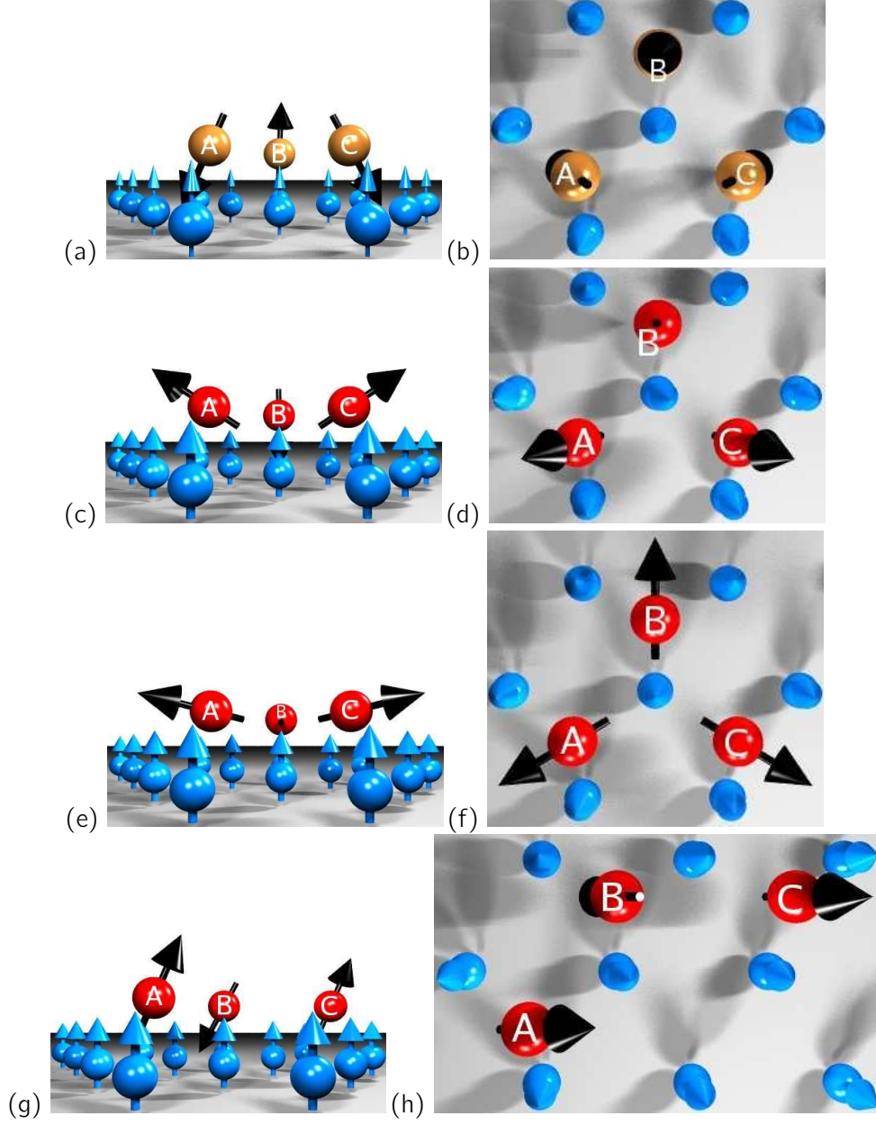
FIG. 13: Side view (a) and top view (b) for the most stable configuration of Cr compact trimer on Ni(111); this corresponds also to the NC1 configuration of the Mn compact trimer. (c) and (d) represent the side view and top view of the ground state (NC2) of Mn compact trimer on Ni(111) while (e) and (f) depict an almost degenerate state (NC3) of the same Mn trimer. Finally, the side view (g) and top view (h) are shown for the most stable configuration of Mn corner trimer on Ni(111). The adatoms are labeled by A, B, and C. Unlabeled atoms (in blue) correspond to the Ni substrate. Reprinted with permission from Ref.[40]. Copyright 2007 by the American Physical Society.
