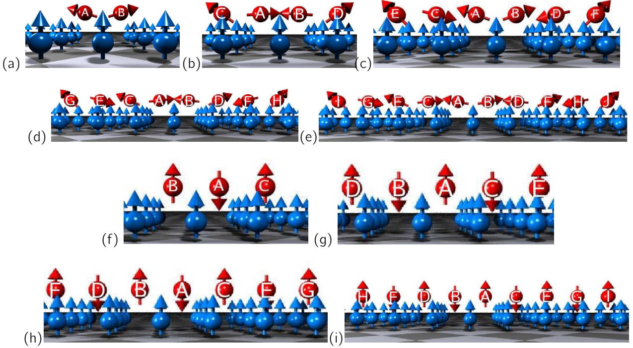
FIG. 7: Magnetic ground configurations of the Mn nanochains on Ni(001) calculated with the KKR method. The nanochains with even number of Mn atoms (2, 4, 6, 8, 10) prefer a non-collinear ground state, the odd ones a collinear one. Atoms in blue correspond to the Ni substrate. Adapted with permission from Ref.[42].
