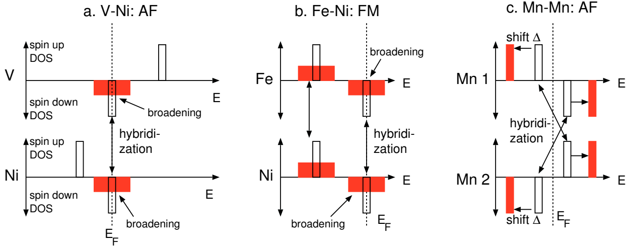
FIG. 5: Alexander-Anderson model for neighboring magnetic atoms: (a) Early 3d transition elements in interaction with Ni surface atoms (double exchange); (b) Late 3d transition elements in interaction with Ni surface atoms (double exchange); (c) Cr or Mn dimer (kinetic exchange). Adapted with permission from Ref.[39].
