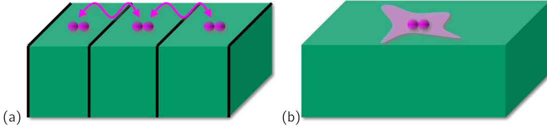
FIG. 3: Adatoms on surface. In (a) the supercell approach is depicted with arrows showing the spurious interaction between nanostructures of adjacent supercells. This unwanted interaction is avoided in the real-space KKR formalism (b).
