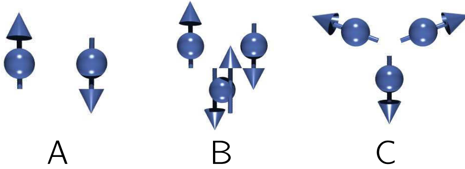
FIG. 1: Example of frustration seen with an antiferromagnetic Cr dimer ( A ) to which we add a third equidistant atom. A magnetically frustrated state is obtained ( B ) because all three atoms tend to couple antiferromagnetically to each other leading then to a non-collinear magnetic structure ( C ) as a ground state.
