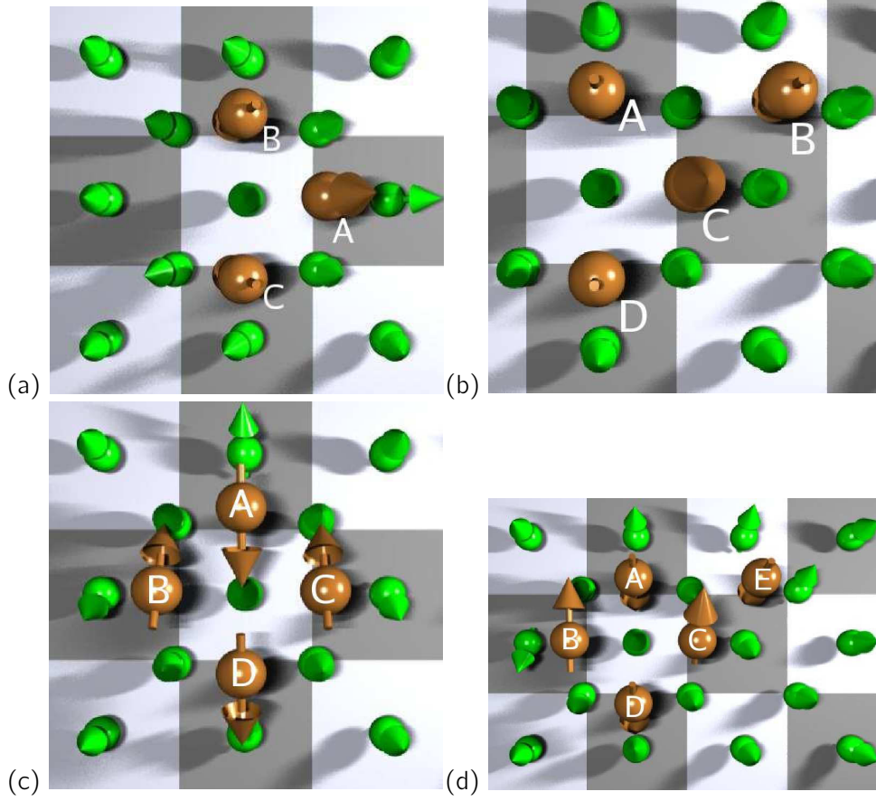
FIG. 10: Front views of complex magnetic states of Cr ad-clusters on \text{Fe}_3\text{ML}/\text{Cu}(001) surface: (i) the trimer is shown in (a), (ii) the T-shape tetramer (tetramer 2) is presented in (b), (iii) the tetramer 1 is depicted in (c) and finally pentamer 1 is shown in (d). Unlabeled atoms (in green) correspond to the Fe substrate. Reprinted with permission from Ref.[41]. Copyright 2008 by the IOPscience.
