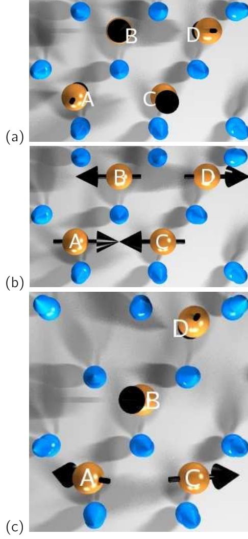
FIG. 14: Top view of the collinear most stable solution (a) and the non-collinear metastable configuration (b) of compact Cr tetramer on Ni(111). In (c) is depicted the Cr tetramer-b magnetic ground state on Ni(111), which basically consists of the non-collinear trimer state of Fig.13(a) coupled antiferromagnetically to the fourth adatom. The adatoms are labeled by A, B, C, and D. Unlabeled atoms (in blue) correspond to the Ni substrate. Reprinted with permission from Ref.[40]. Copyright 2007 by the American Physical Society.
