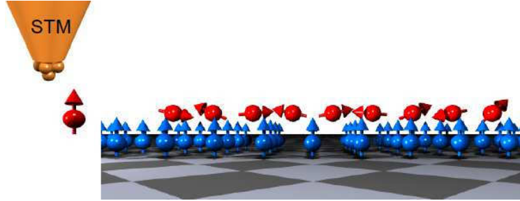
FIG. 2: A STM tip moving an adatom towards a nanochain.
