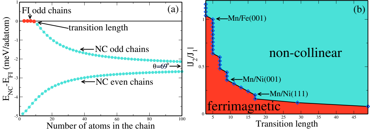
FIG. 8: (a) Energy differences obtained from the Heisenberg model between the NC and the FI configuration for different lengths of Mn chains on Ni(001). The parameters used were J_1 = -138 meV and J_2 = 52 meV. (b) Magnetic phase diagram of the odd chains showing the effect of the ratio J_2/J_1 on the transition lengths. If the length of the chains is smaller than the transition length, the FI configuration is the ground state. Adapted with permission from Ref.[42].
