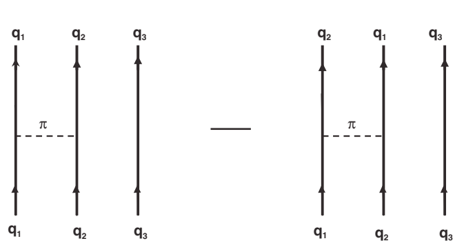
FIG. 3. Second order \pi -meson exchange diagrams.
