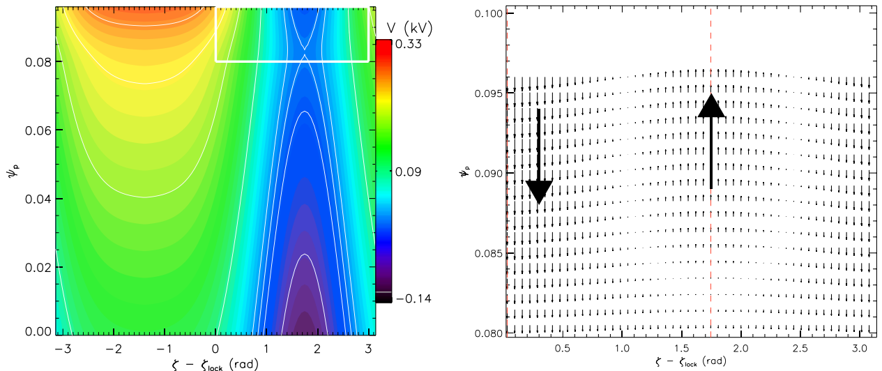
FIG. 8. (a) Contour plot of the model of potential, in the 0/1 symmetry. The phase has been chosen as \zeta_0 = 3/2\pi , in order to match the experimental data. The white inset encloses the region of the convective cell measured by the GPI diagnostic, shown in Fig. 2; (b) By differentiating the potential, we get the electric field in the plane perpendicular to \vec{B} , with its two components (E^\zeta, E^r) . Note that the region of E^r > 0 corresponds to the center of the cell, or, equivalently, to the potential well.
