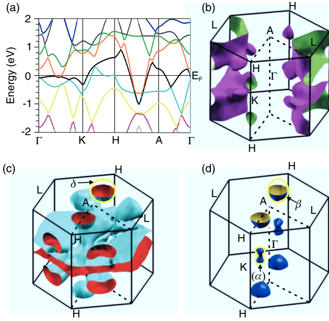
FIG. 4. (Color) Calculated electronic structure of \text{CrB}_2 with a cycloidal magnetic ordering wave vector \mathbf{q} = 0.3 \mathbf{q}_{110} using the WIEN2K package. (a) Band structure of \text{CrB}_2 around the Fermi level E_F . In total, three bands (blue, orange, black) cross E_F . (b)–(d) Fermi surface sheets of \text{CrB}_2 corresponding to the three bands that cross E_F in (a). For clarity, the Fermi surface sheets corresponding to the three different bands are plotted separately. (b) The Fermi surface sheet corresponding to the blue band consists of a singly connected structure centered around the L point at the boundary of the first Brillouin zone. It has predominantly Cr- d character. (c) Fermi surface corresponding to the black band. Two ball-shaped, B- p derived Fermi surface pockets are present between the A and the H points. The extremal orbit \delta assigned to the experimentally observed dHvA frequency is shown in yellow. The ball shape of this pocket is quite insensitive to magnetic order (see main text). The remaining Fermi surface sheets of this band exhibit a complicated structure and are of Cr- d character. Thorough analysis with SKEAF showed that none of the numerous further extremal orbits of these sheets are close to the experimental ones. (d) Two ball-shaped and two dumbbell-shaped Fermi surface pockets originate from the orange band in (a). The orbit \beta is allocated to the ball-shaped pocket as indicated. This pocket is also predominantly B- p like and very insensitive to the magnetic order. The dumbbell-shaped pockets have Cr- d orbital character. The frequency of the \alpha orbit seen in the experiment matches reasonably well to this pocket (see Table I), while the angular dependence does not. In light of the fact that the pocket is of Cr- d orbital character and thus very sensitive to the exact form of the magnetic order, we refrain from a clear assignment.
